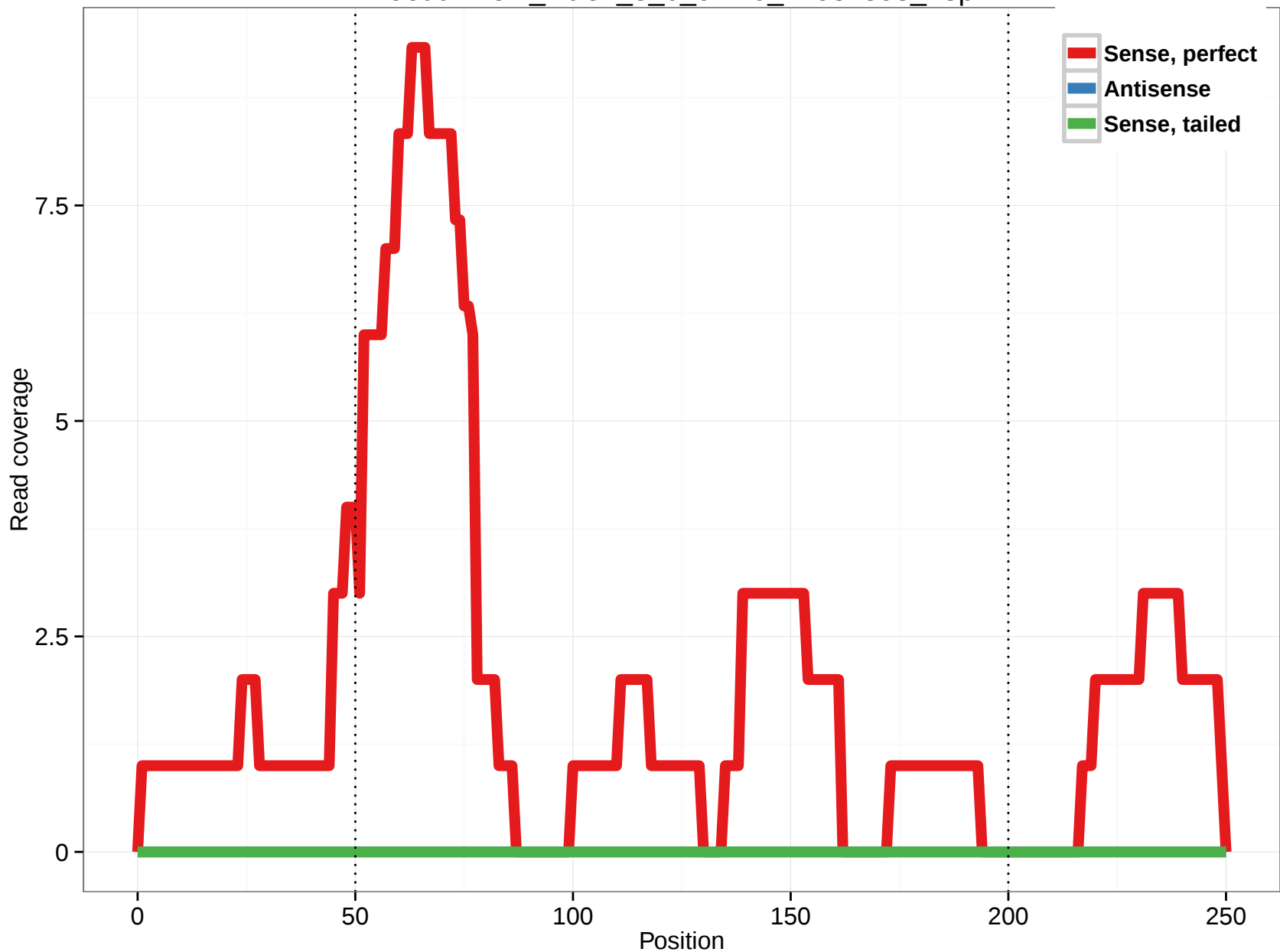
uc002xro.2_intron_8_0_chr20_44987598_r.3p
