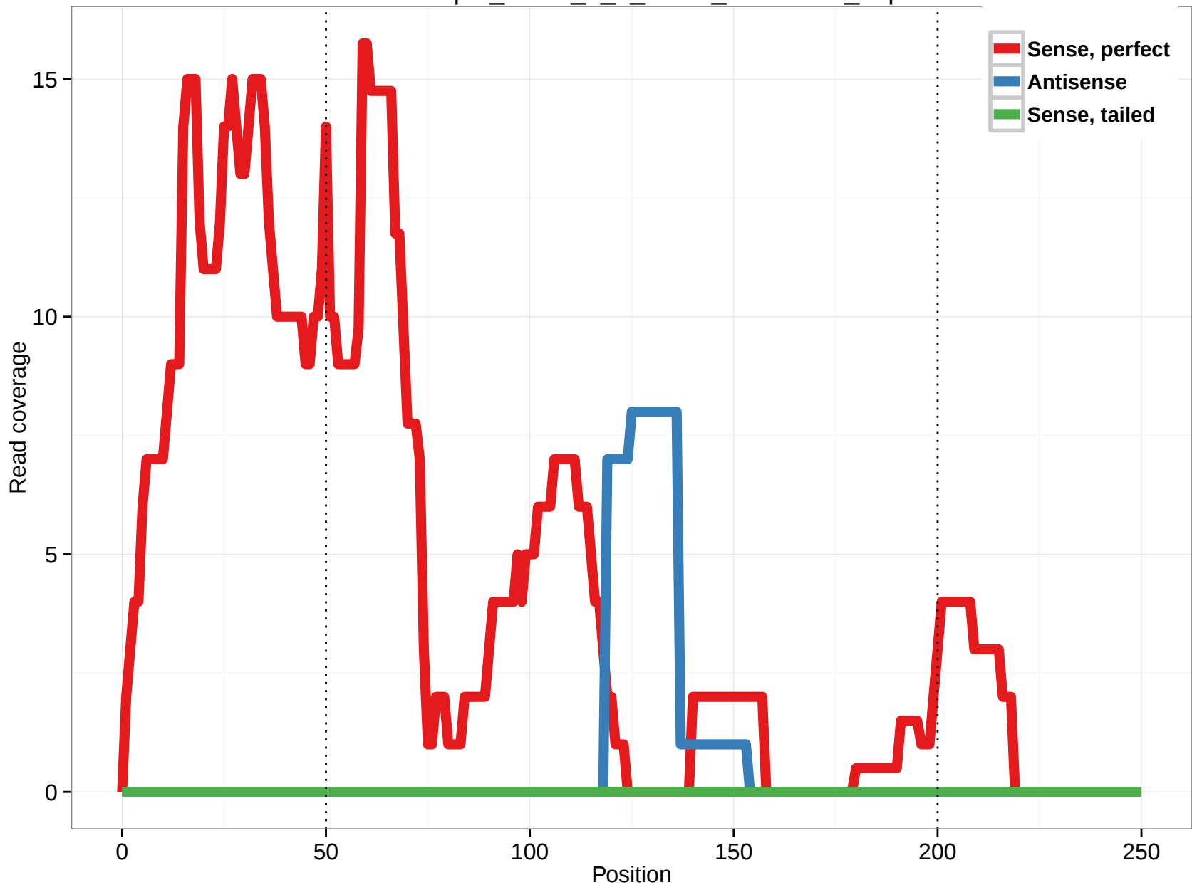
uc002xfp.2_intron_0_0_chr20_35234469_f.5p
