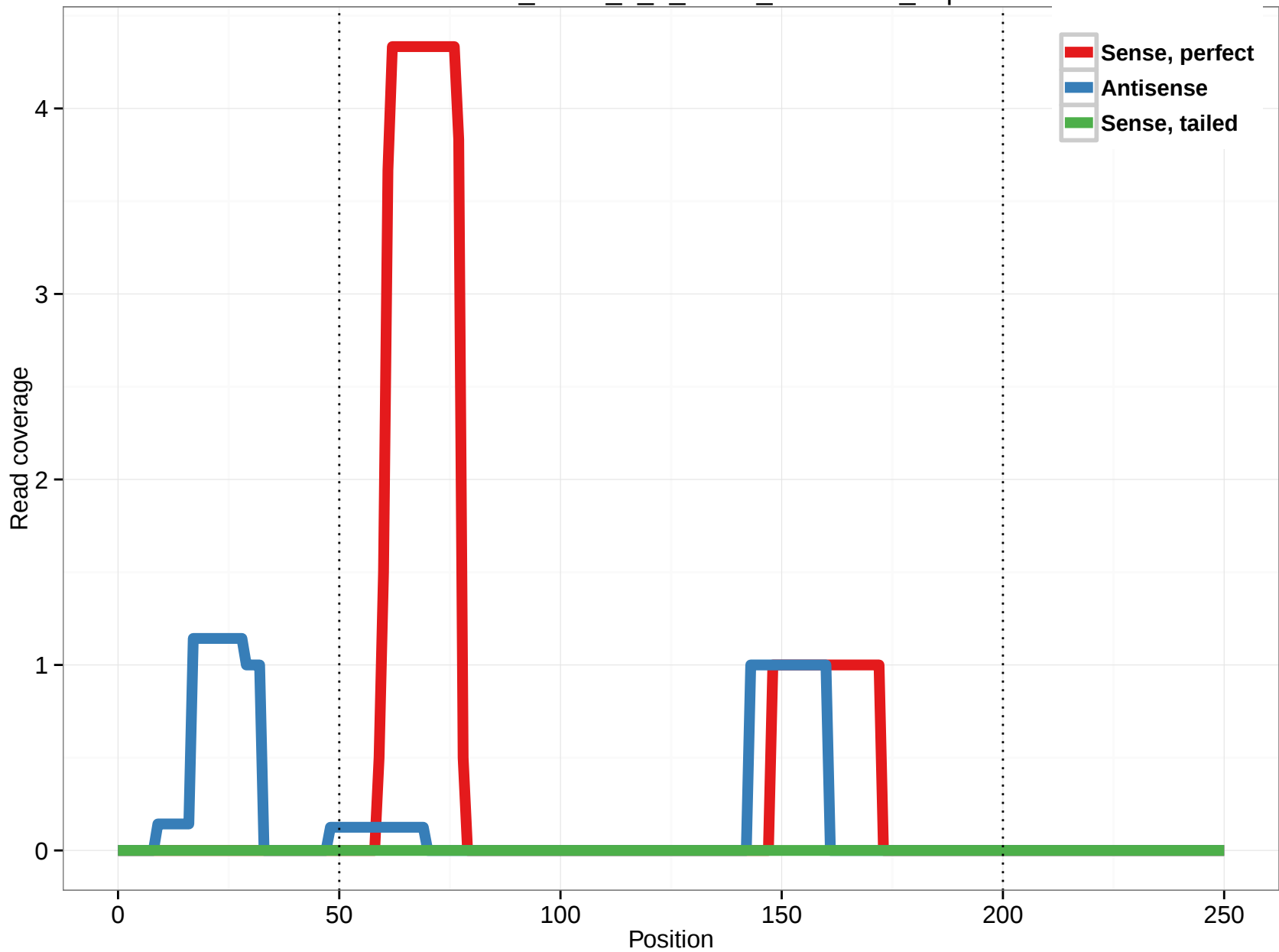
uc002xer.1_intron_6_0_chr20_34575456_f.3p
