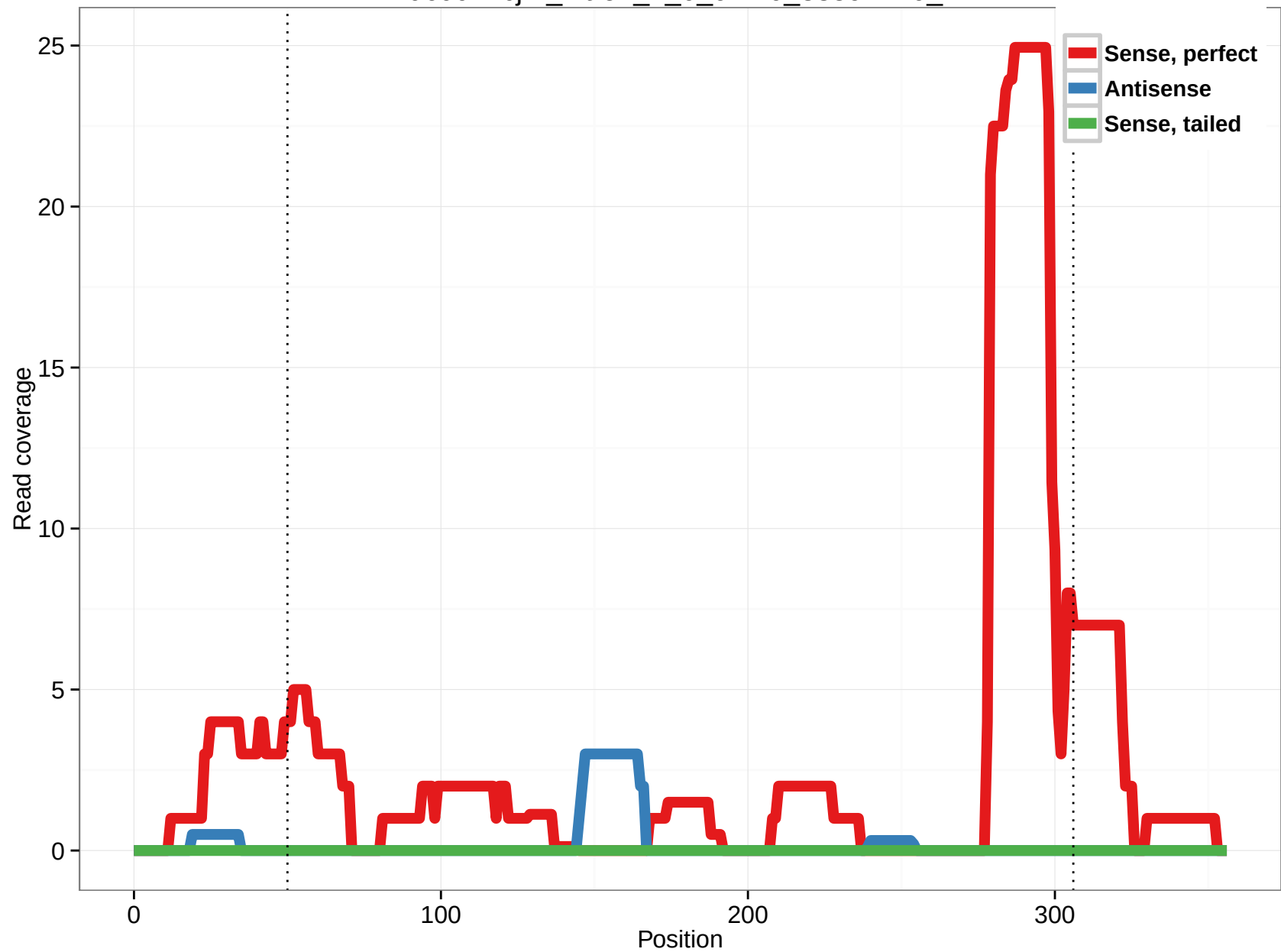
uc002xbj.2_intron_1_0_chr20_33591420_r
