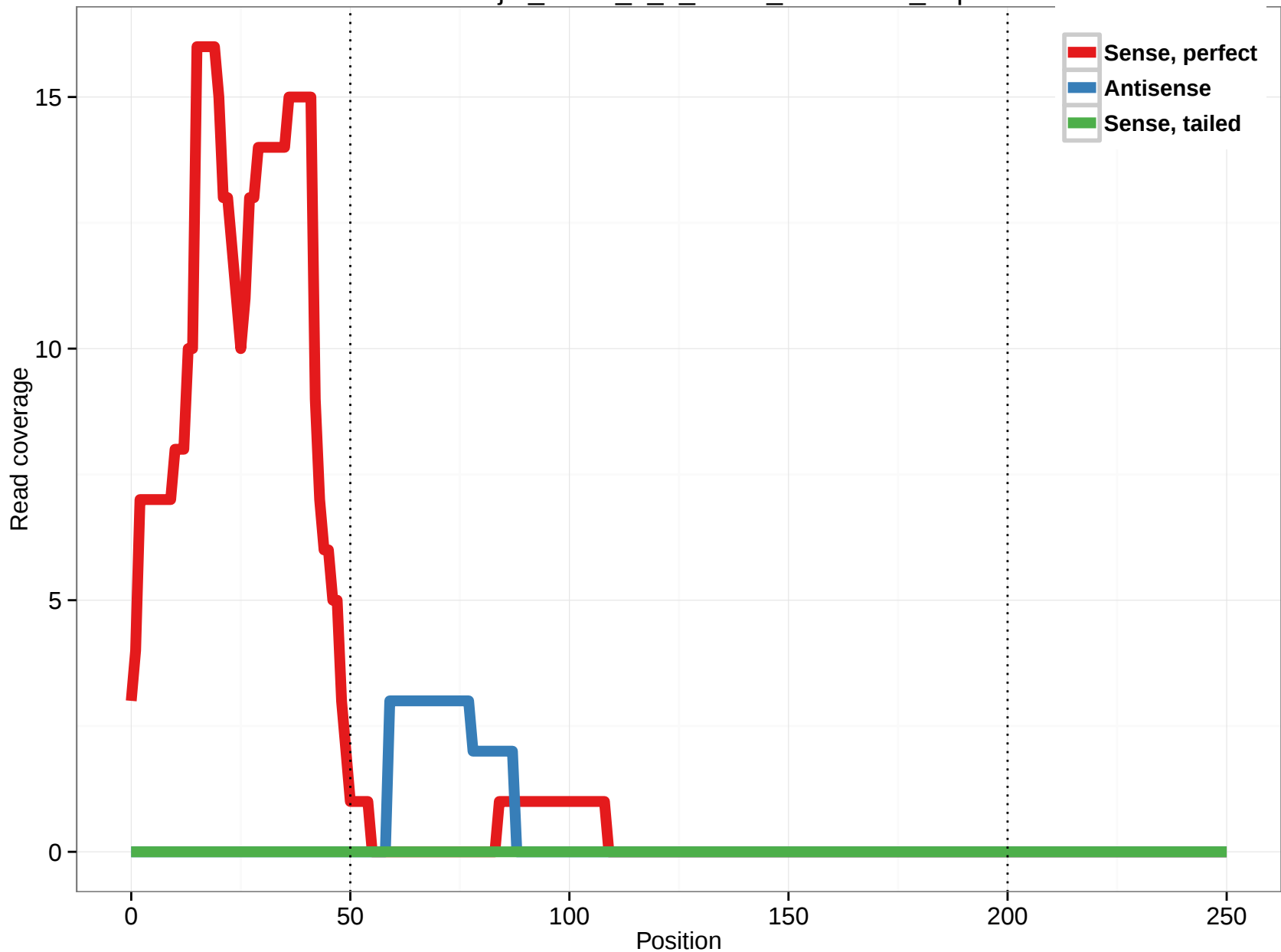
uc002wxj.2_intron_8_0_chr20_30734659_f.5p
