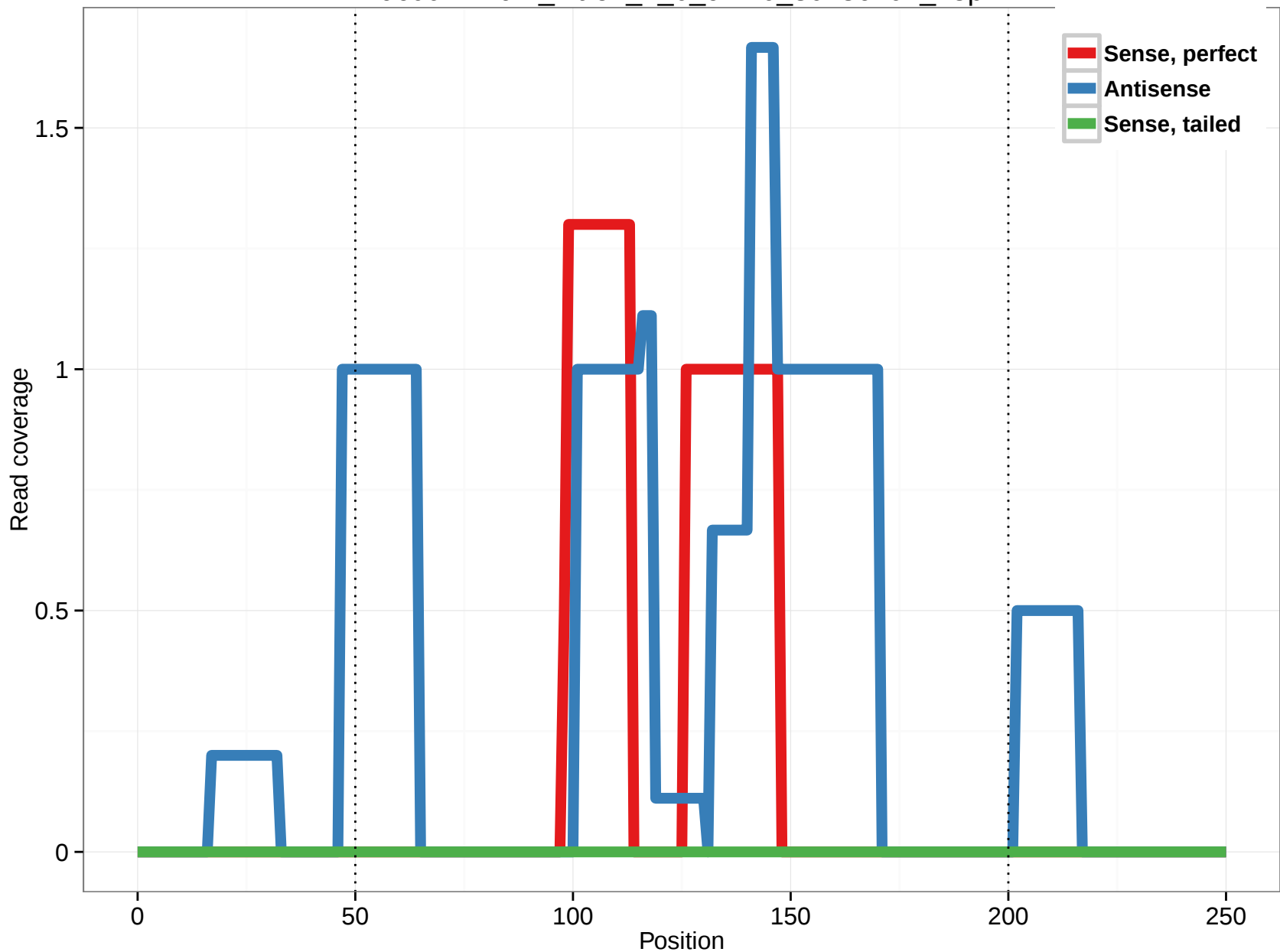
uc002wwwu.1_intron_1_0_chr20_30436707_r.5p
