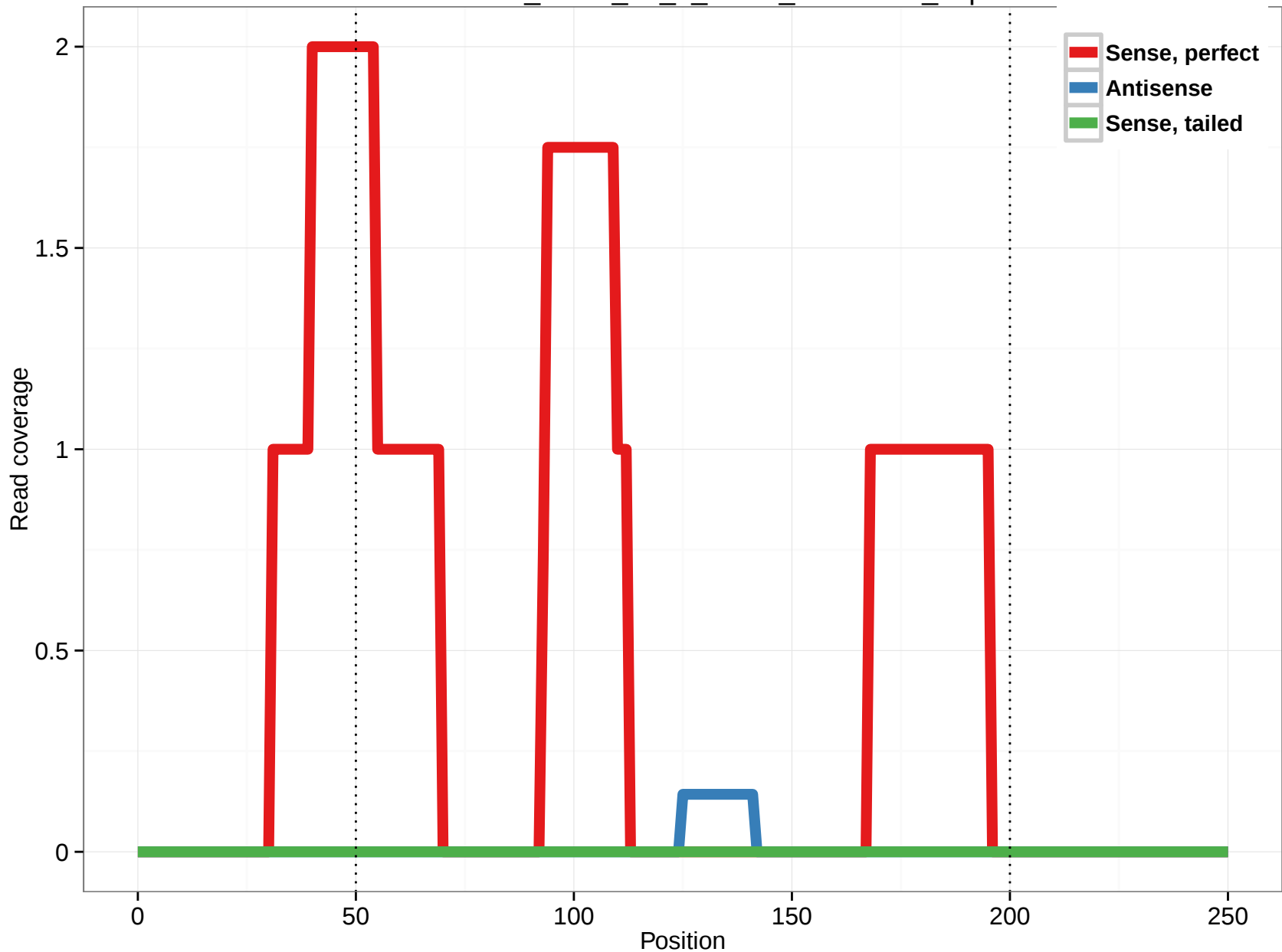
uc002wsf.1_intron_13_0_chr20_21319727_f.3p
