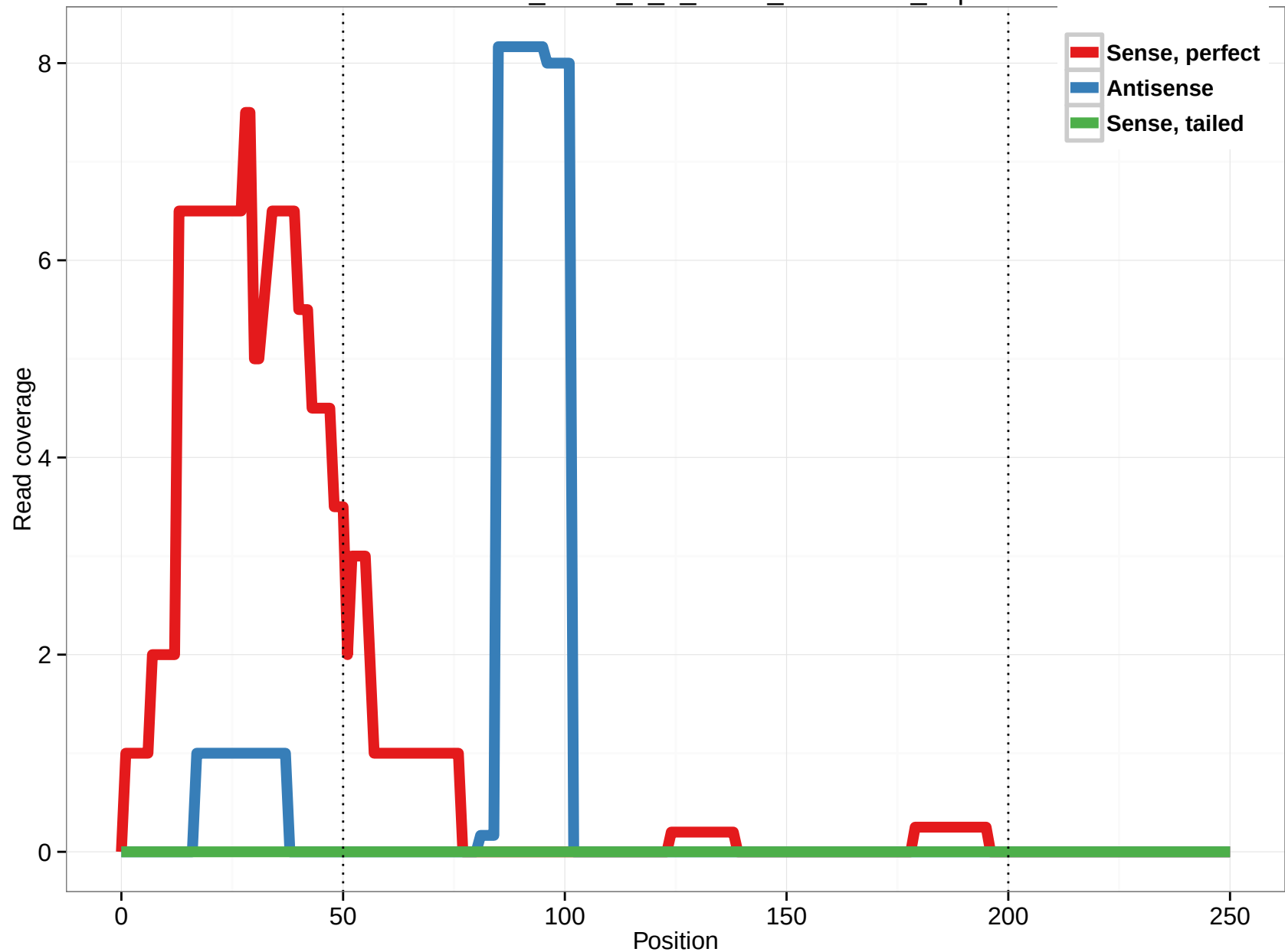
uc002wsb.2_intron_0_0_chr20_21106846_f.5p
