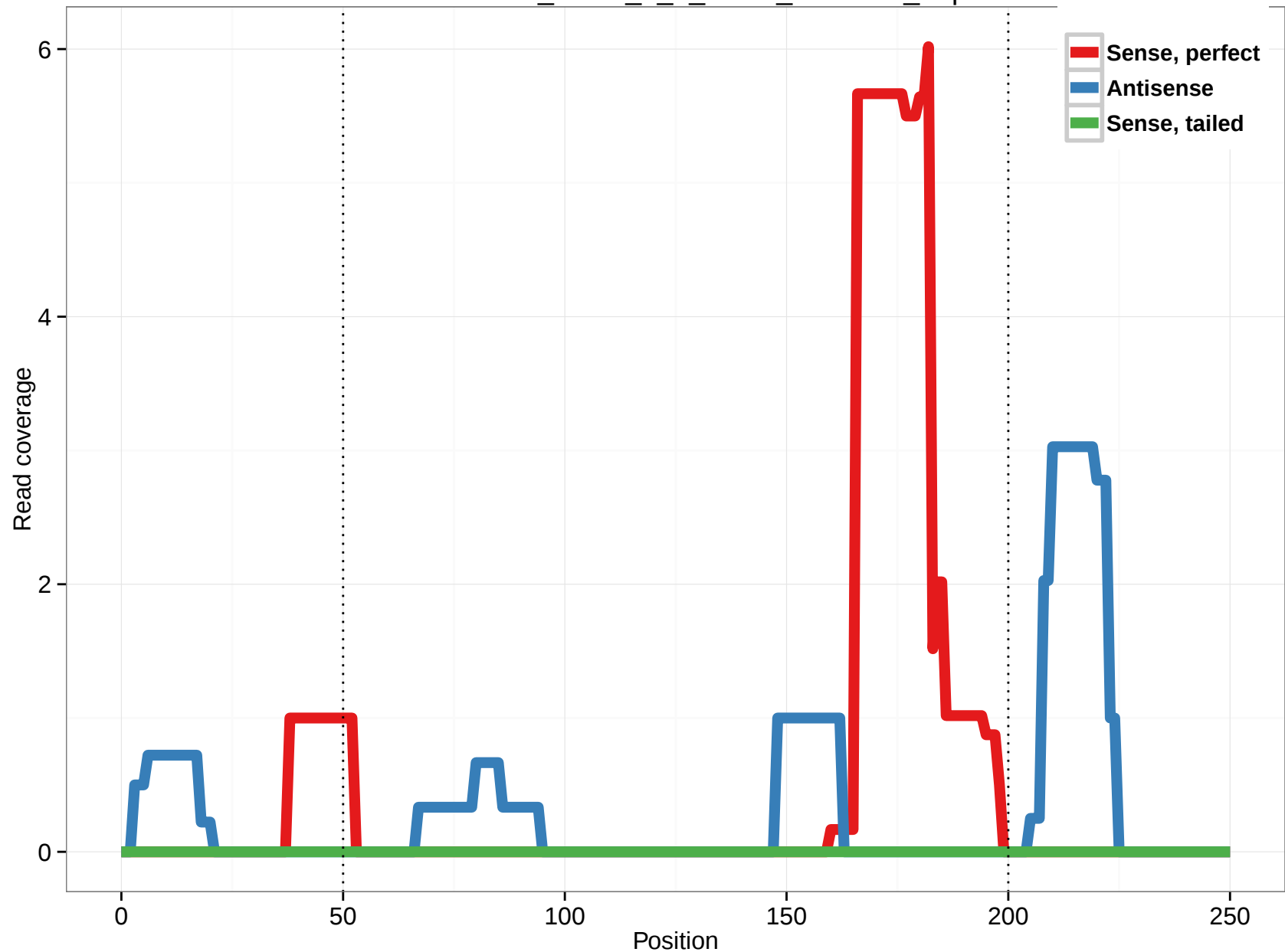
uc002whu.2_intron_1_0_chr20_3063825_r.3p
