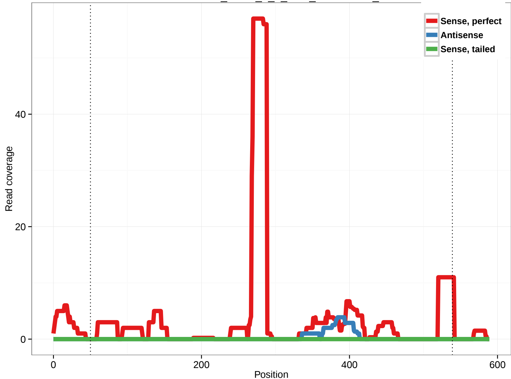
uc002wcc.1_intron_3_0_chr2_242650904_f
