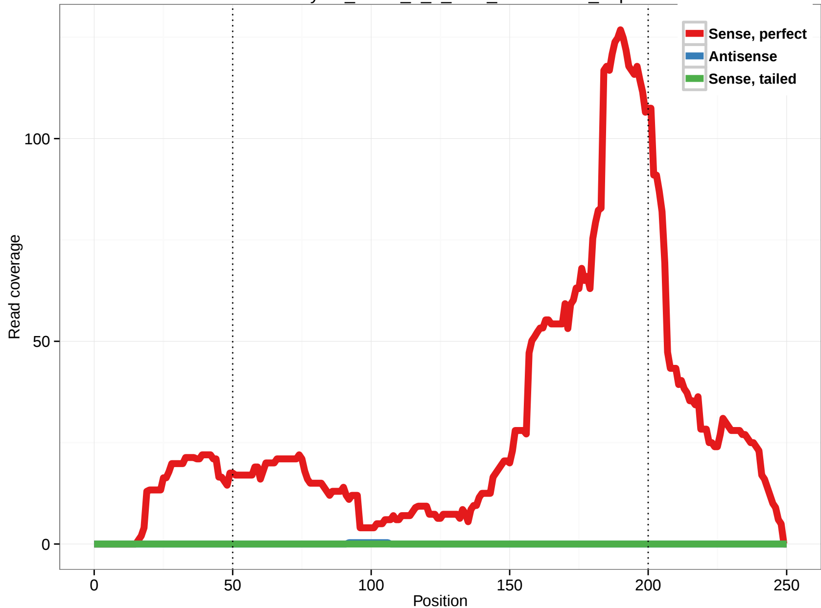
uc002vyu.1_intron_1_0_chr2_241069446_r.5p
