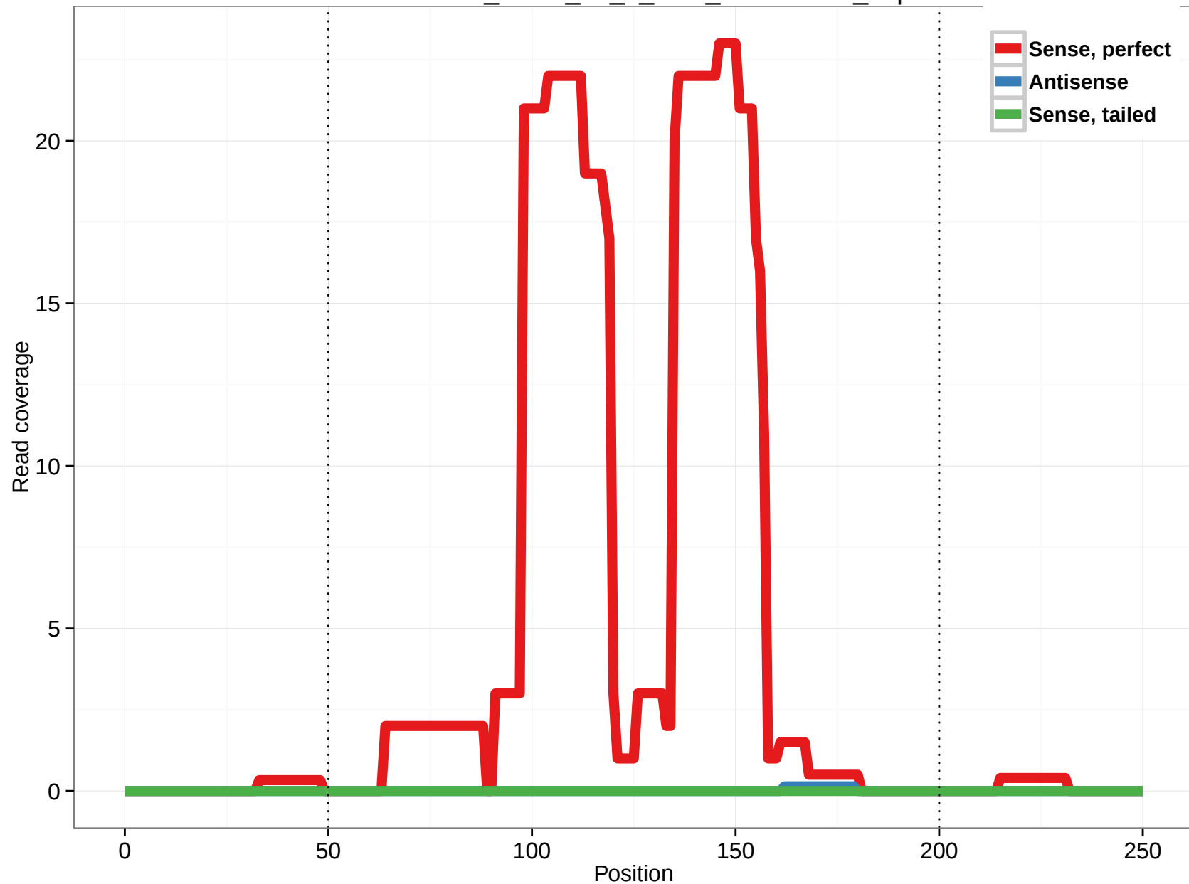
uc002vui.1_intron_25_0_chr2_234371382_f.3p
