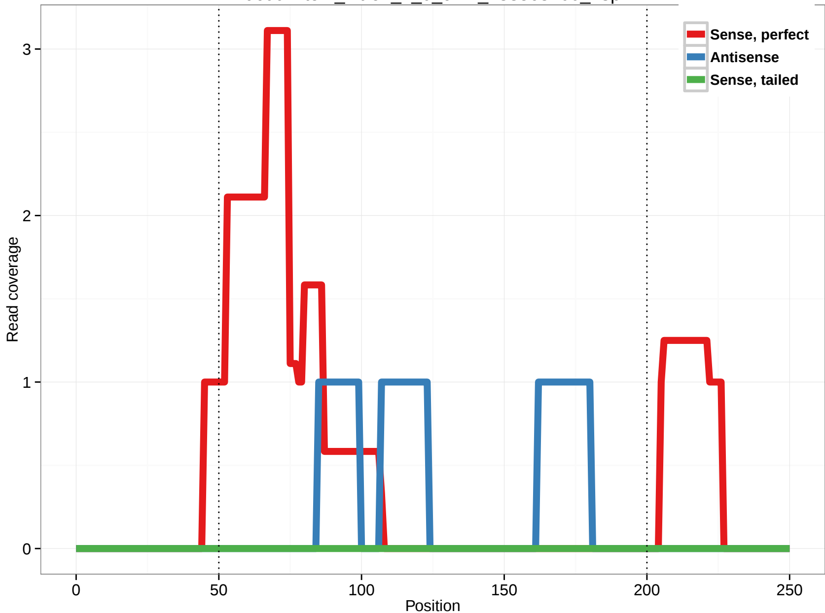
uc002vte.2_intron_2_0_chr2_233568200_f.3p
