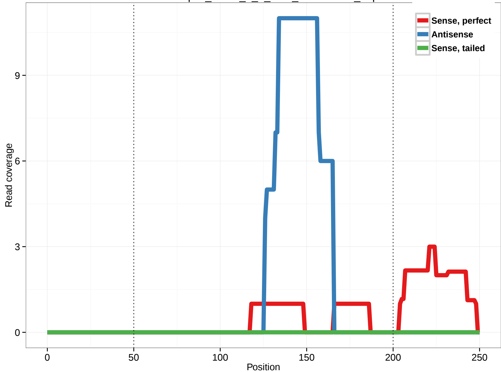
uc002vqx.2_intron_5_0_chr2_231675038_f.3p
