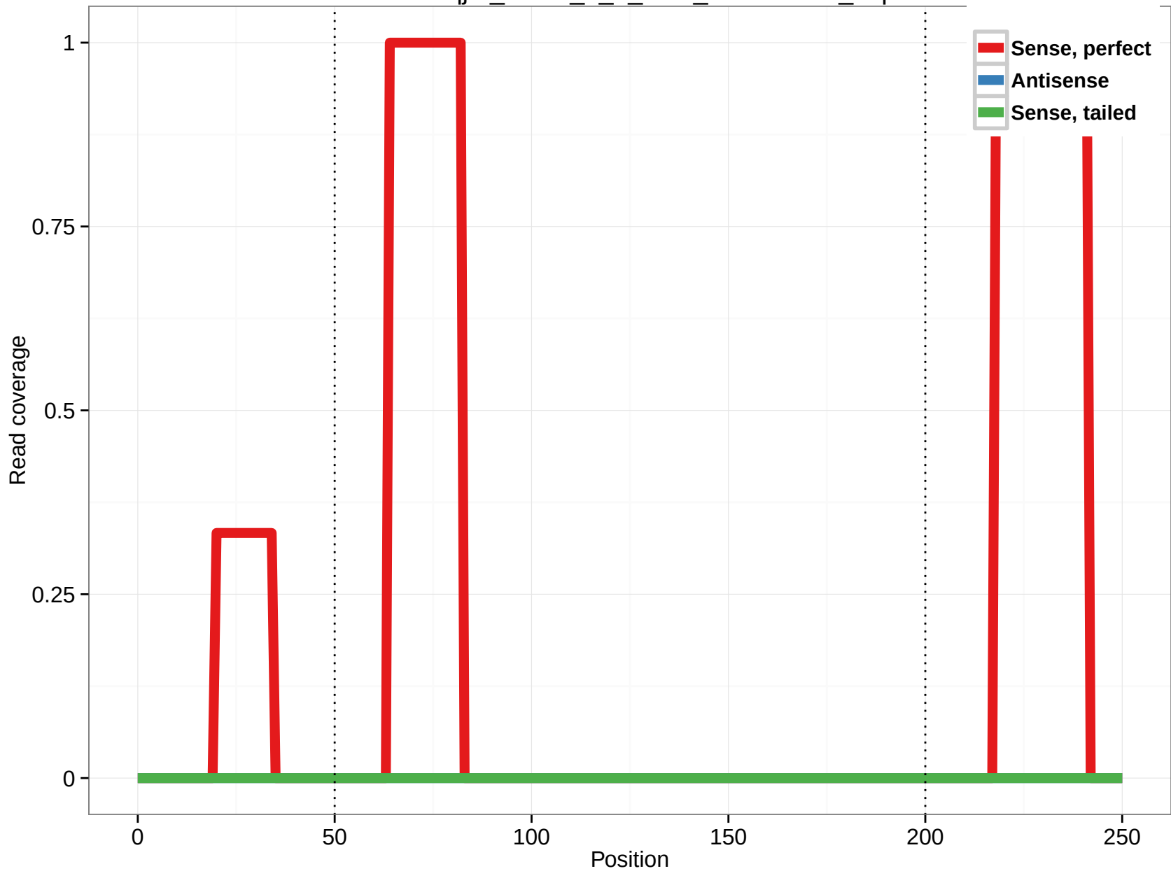
uc002vqj.2_intron_1_0_chr2_231101976_f.5p
