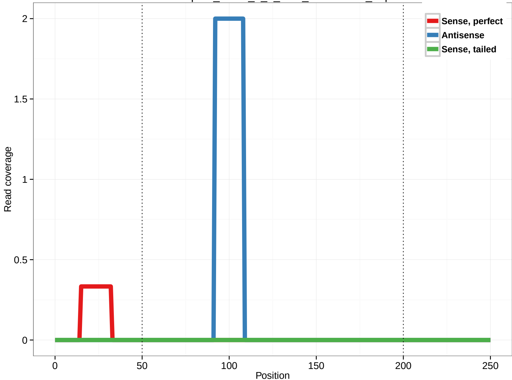
uc002vph.2_intron_0_0_chr2_228476373_r.5p
