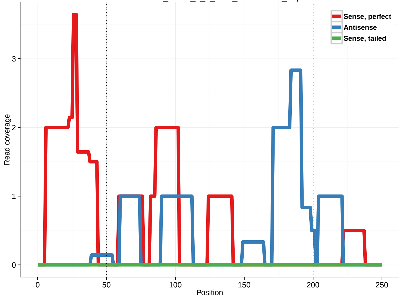
uc002vos.2_intron_0_0_chr2_228190144_f.5p
