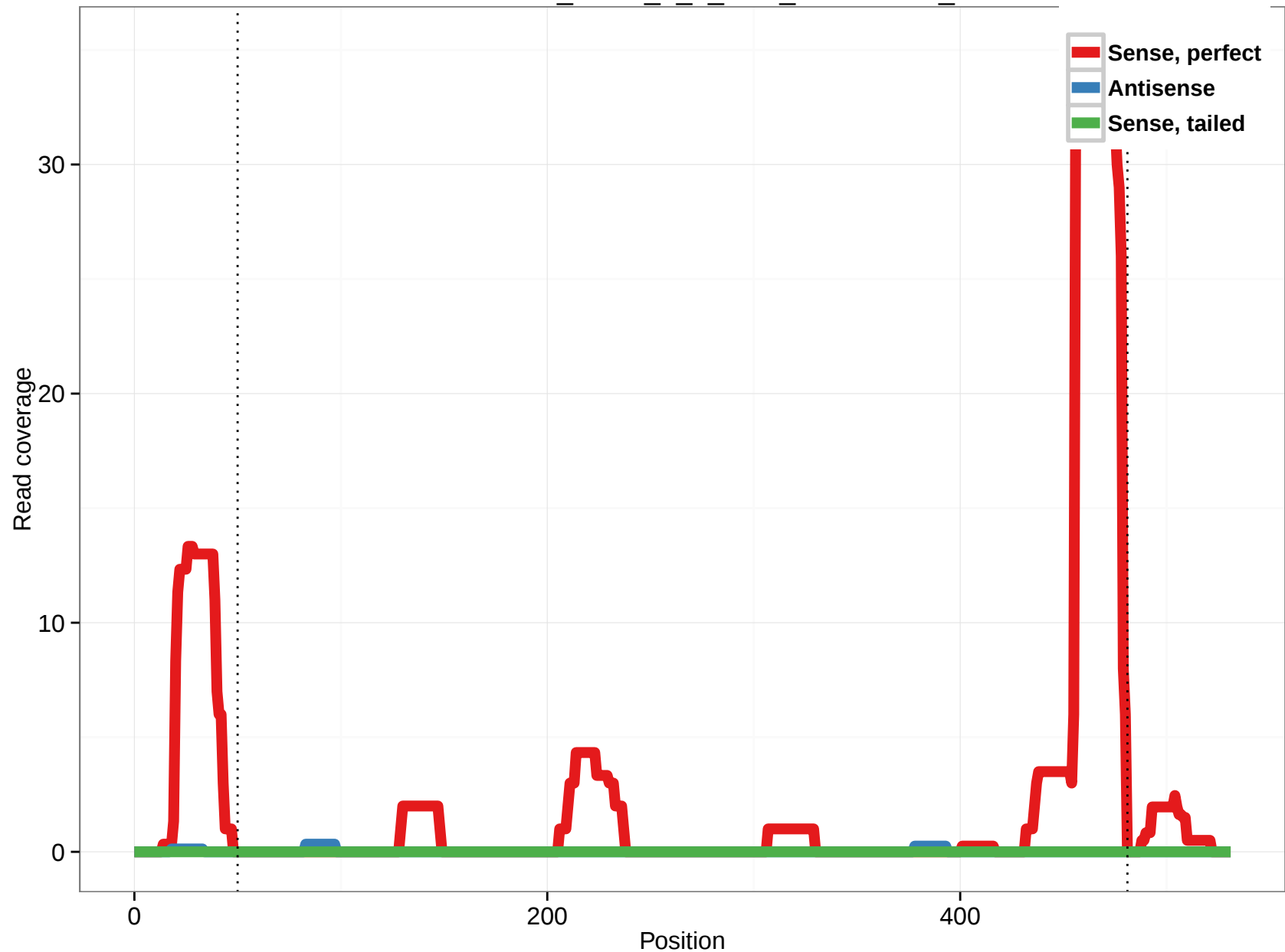
uc002vmo.3_intron_7_0_chr2_220497165_f
