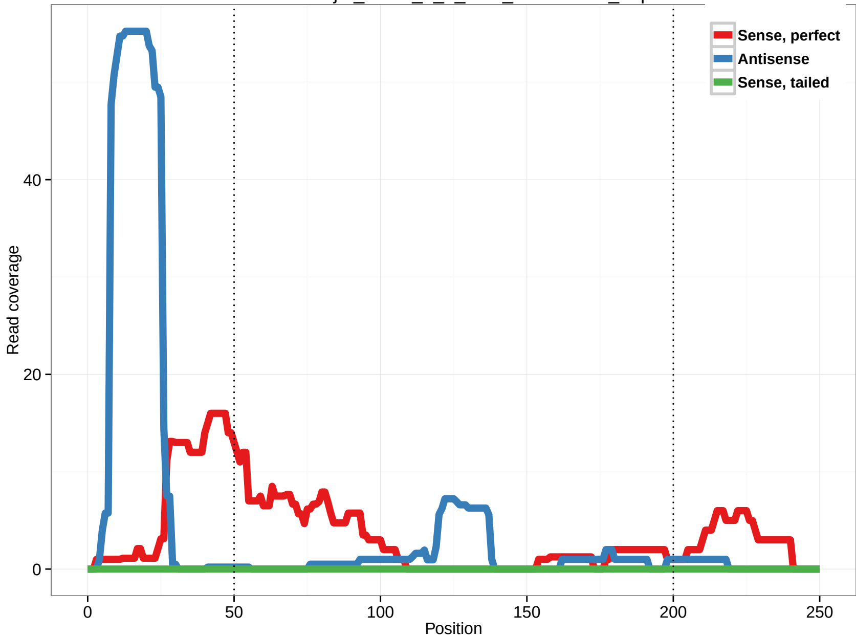
uc002vmj.2_intron_7_0_chr2_220433047_r.5p
