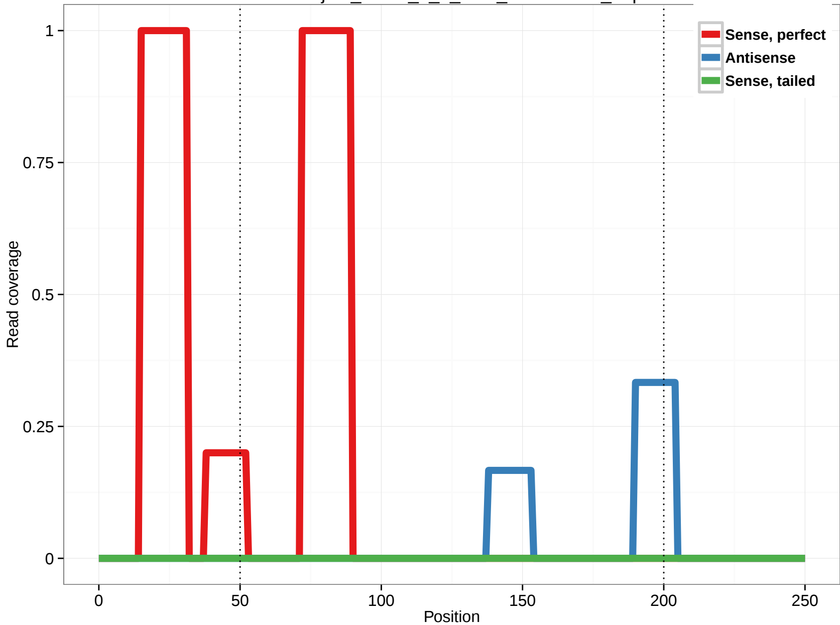
uc002vjb.1_intron_9_0_chr2_219693324_r.3p
