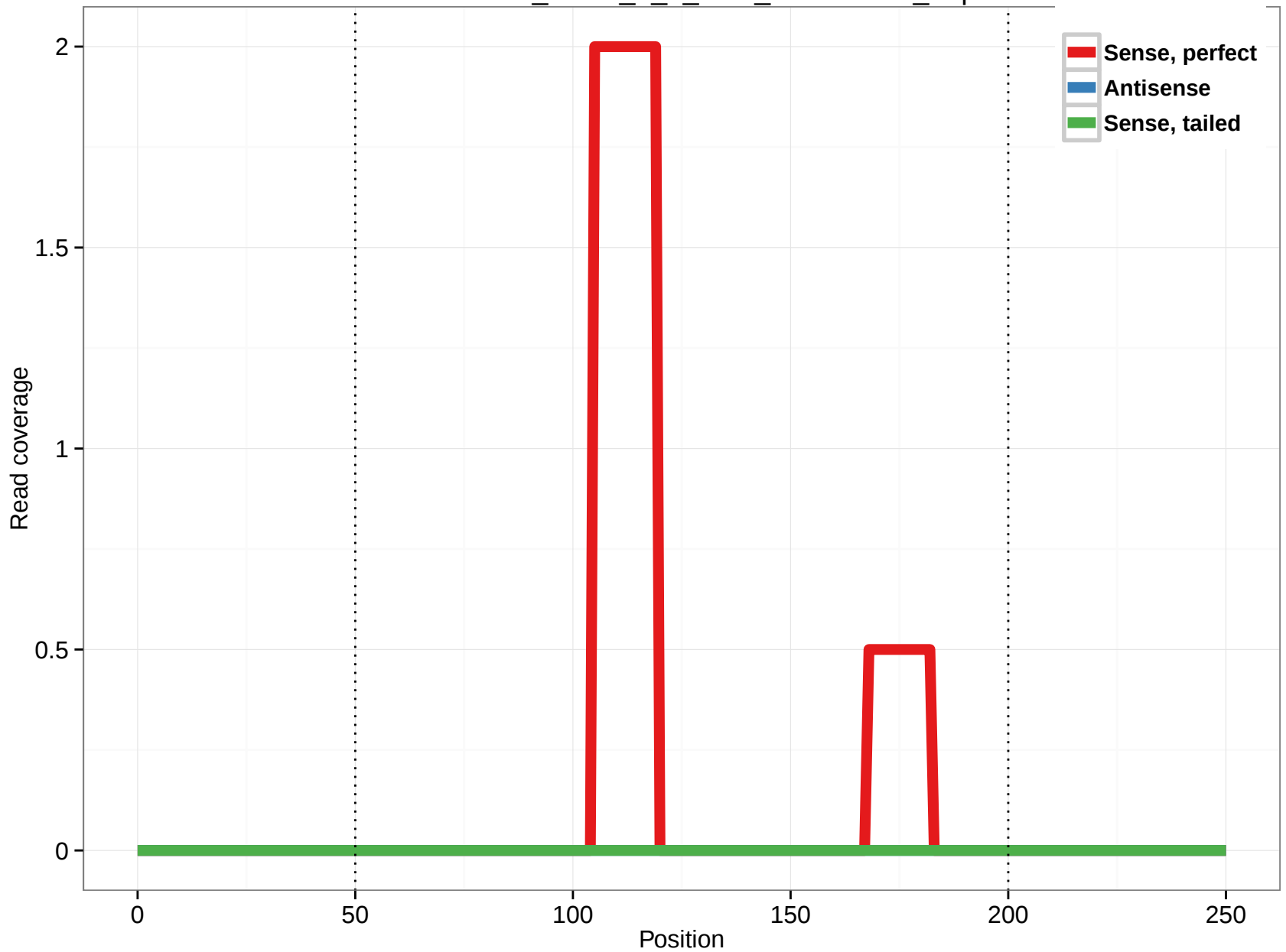
uc002veb.2_intron_4_0_chr2_211163288_r.3p
