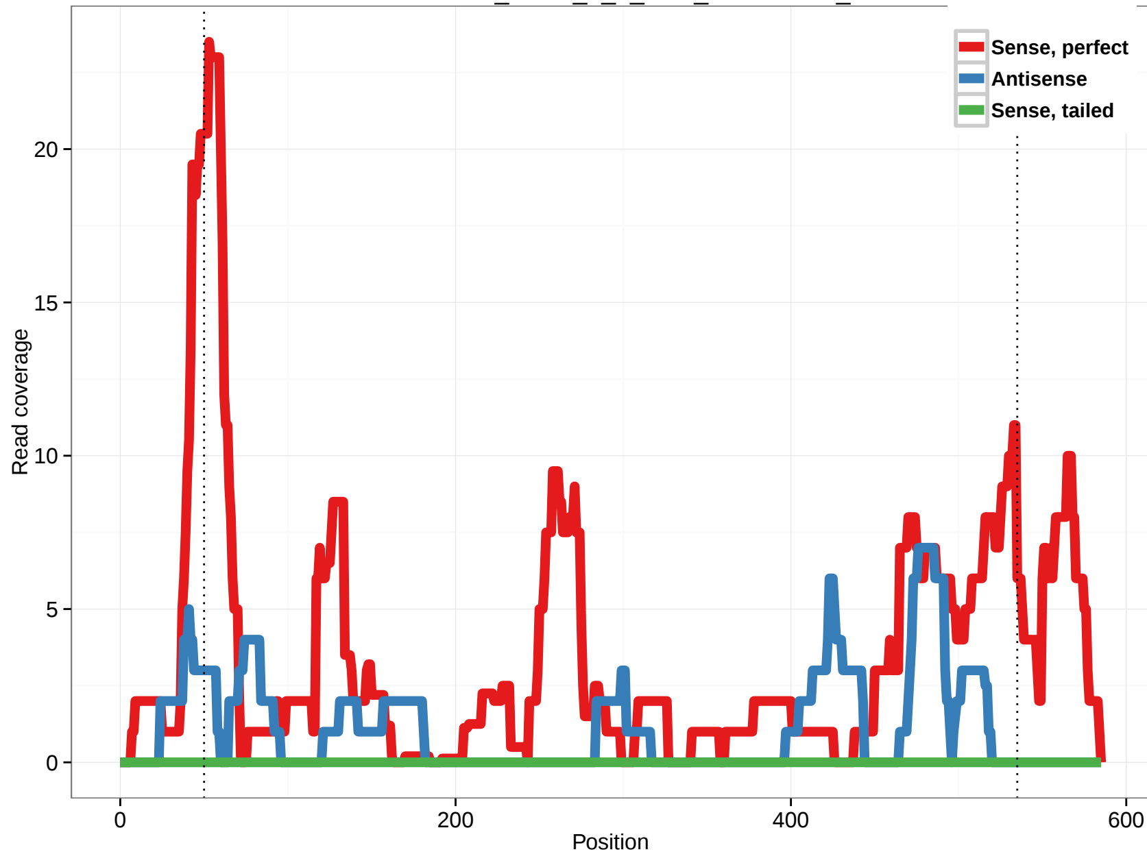
uc002usb.2_intron_0_0_chr2_191514087_f
