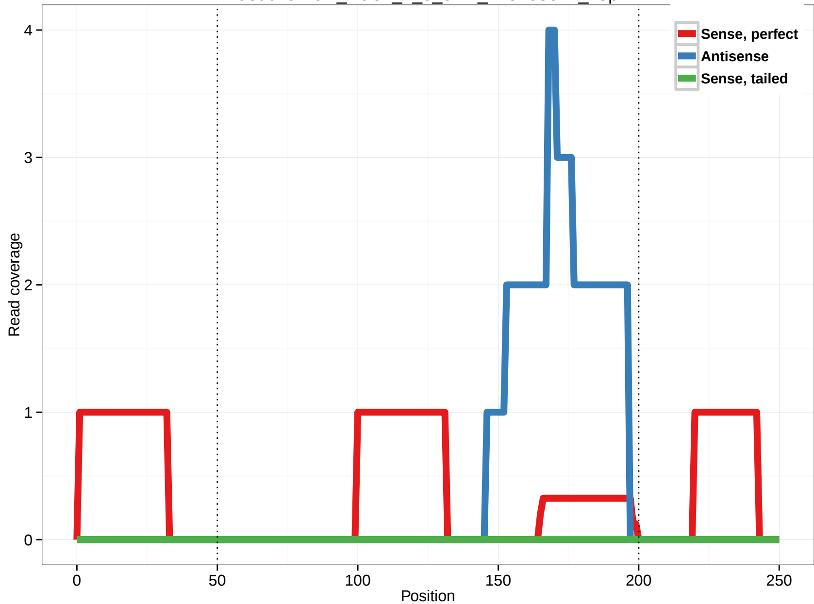
uc002umb.1_intron_2_0_chr2_179295617_f.5p
