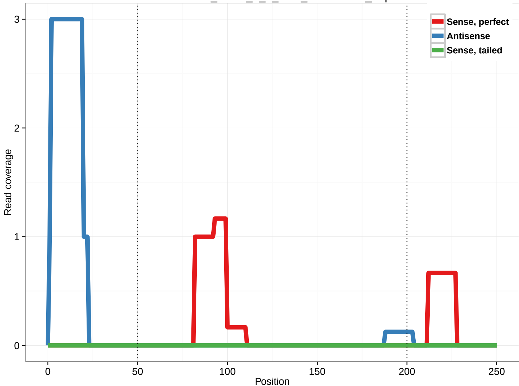
uc002uht.2_intron_1_0_chr2_173599162_r.5p
