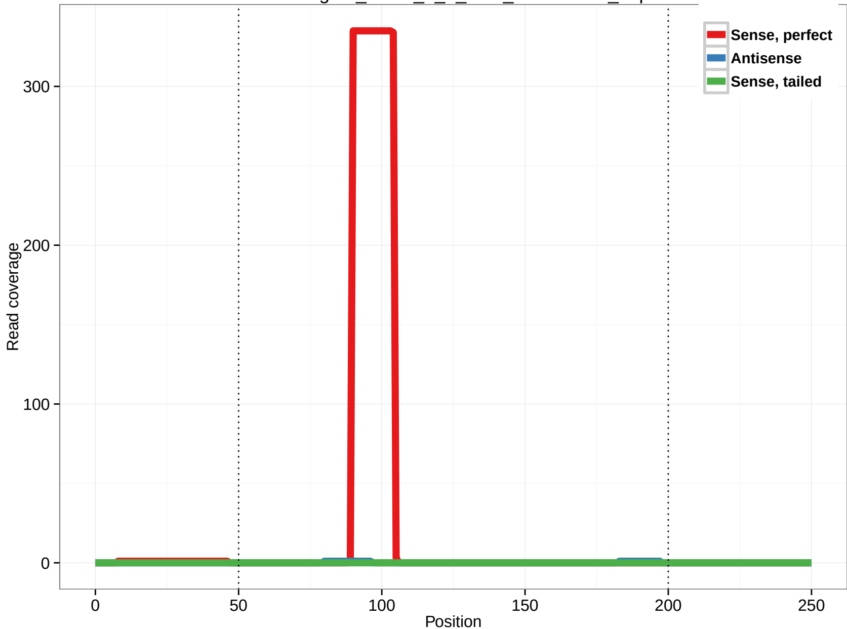
uc002ugh.2_intron_2_0_chr2_171678660_f.5p
