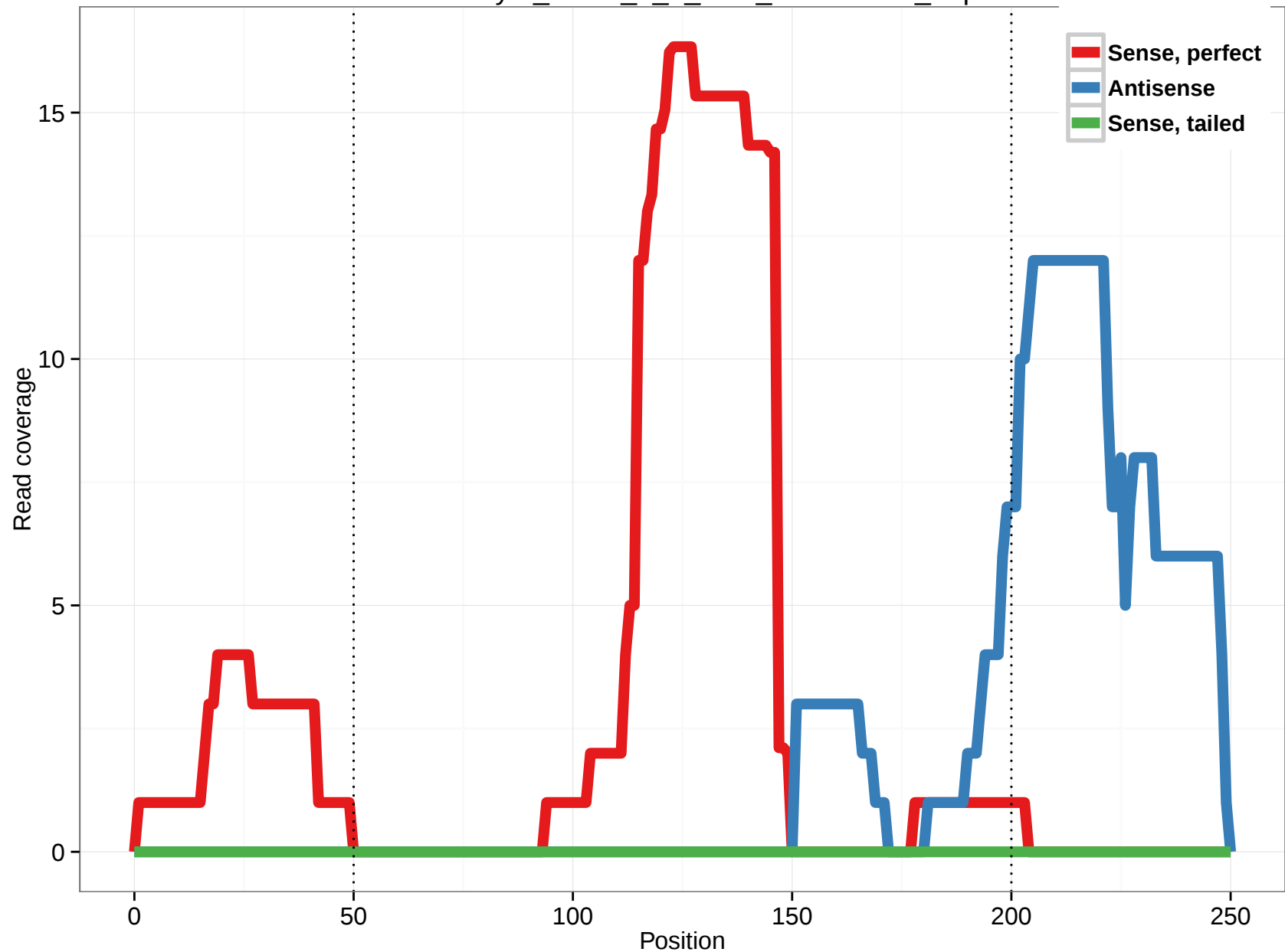
uc002uey.2_intron_1_0_chr2_170419861_r.5p
