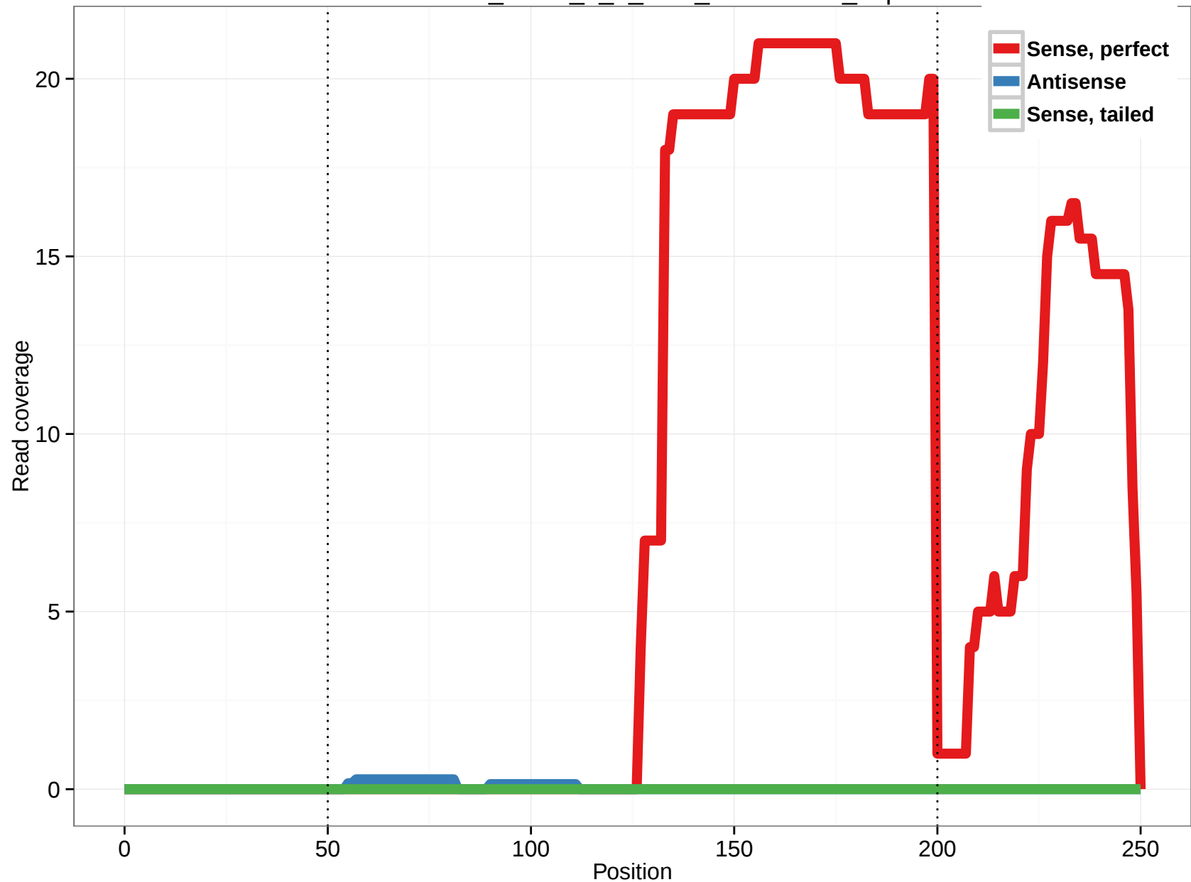
uc002tur.2_intron_7_0_chr2_136528306_f.3p
