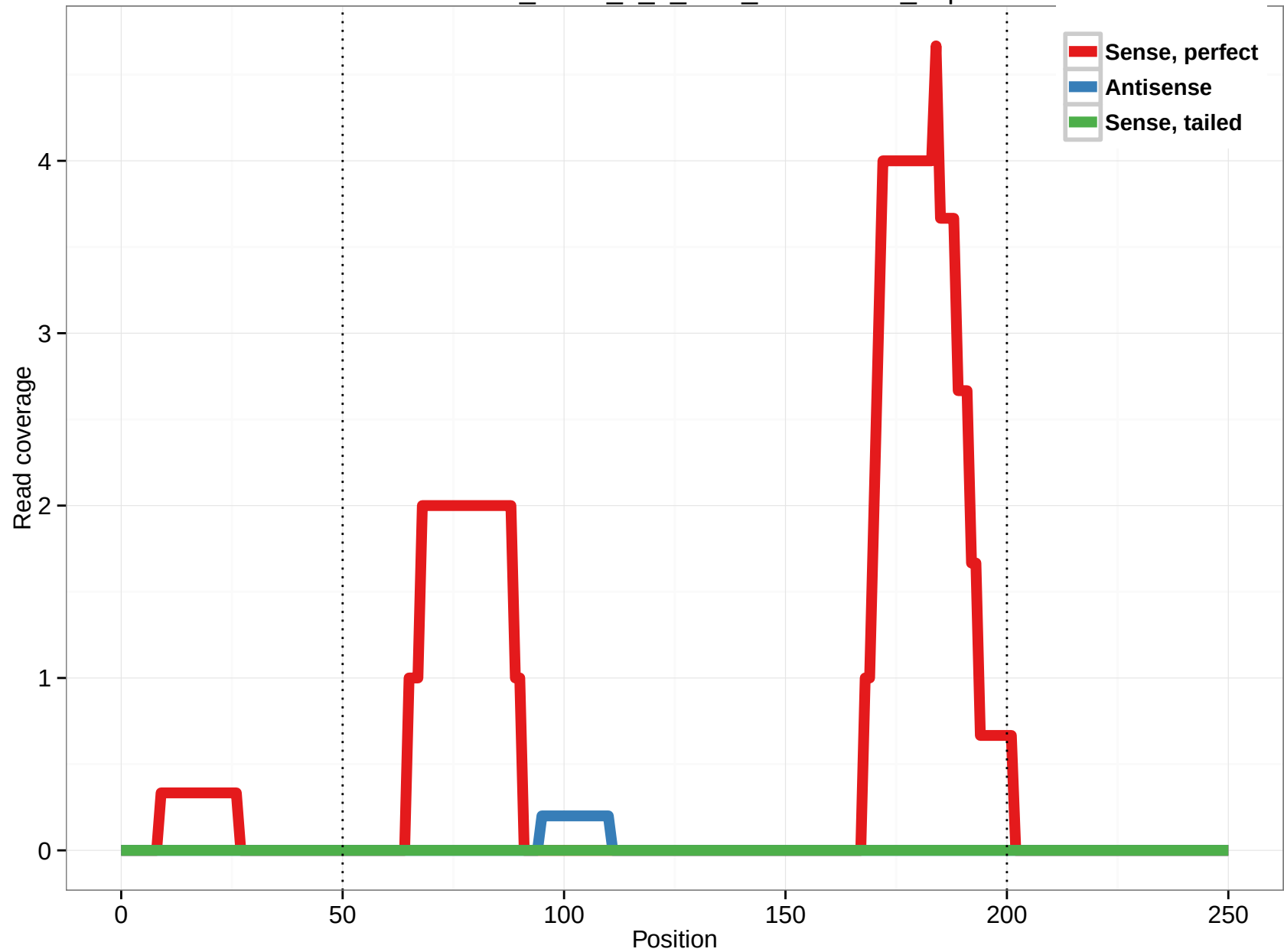
uc002tur.2_intron_1_0_chr2_136505940_f.3p
