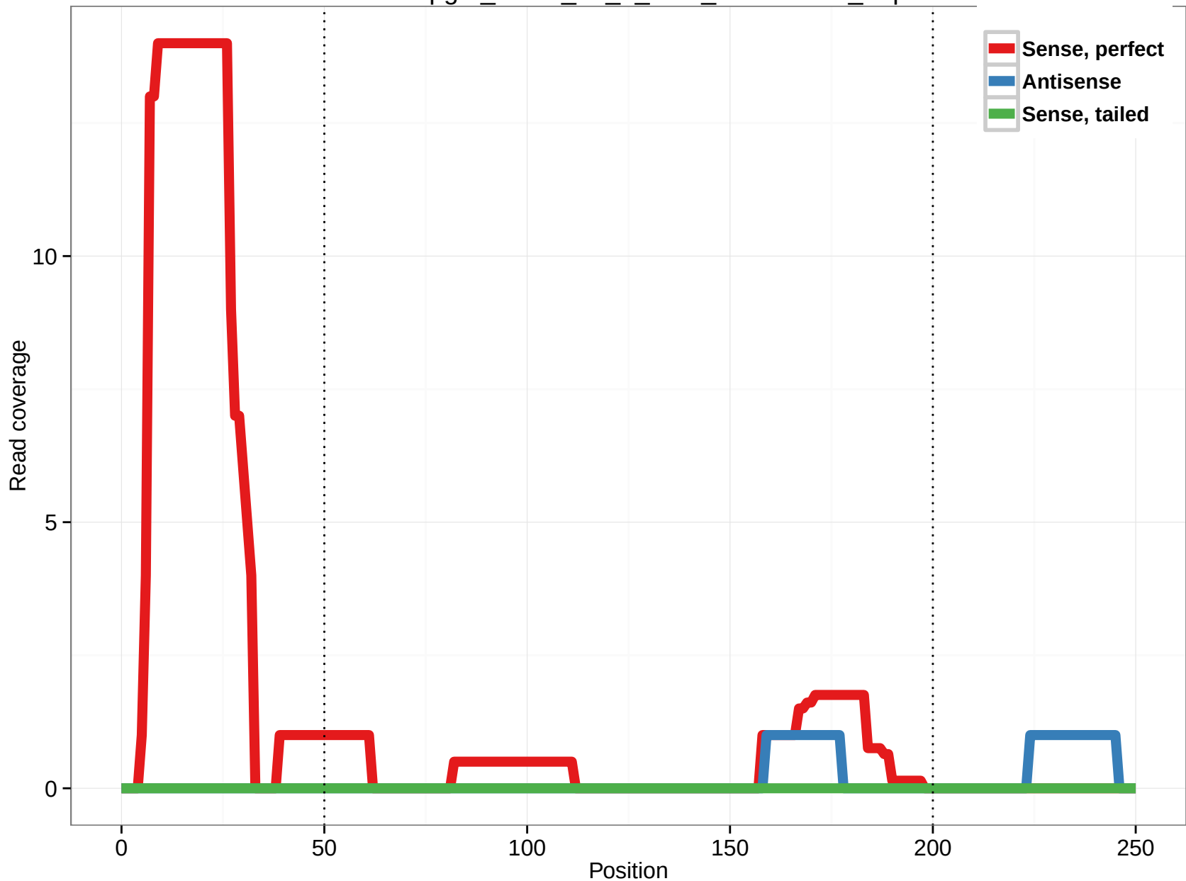
uc002tpg.1_intron_19_0_chr2_128526576_r.5p
