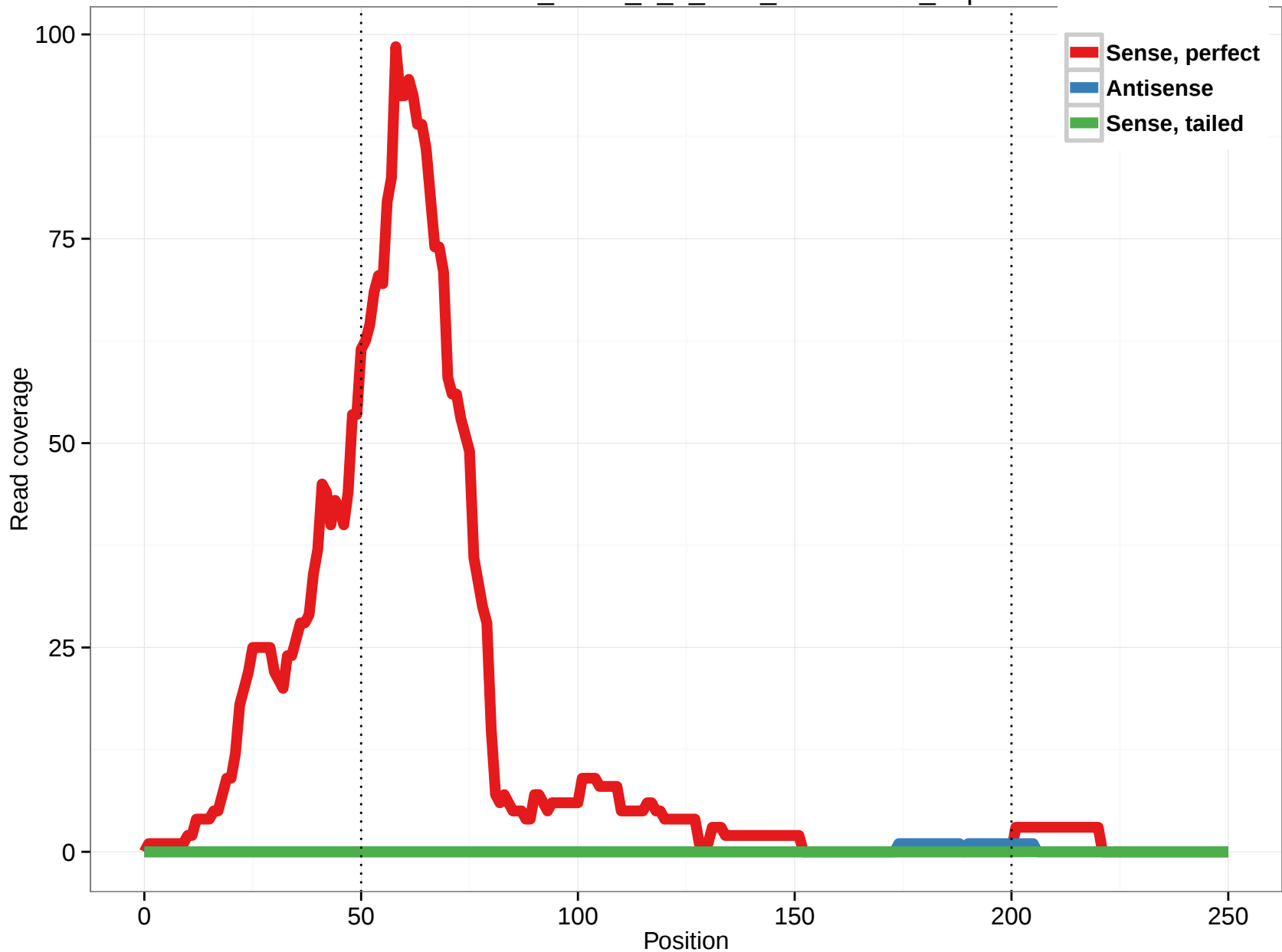
uc002tmc.1_intron_0_0_chr2_120436802_f.5p
