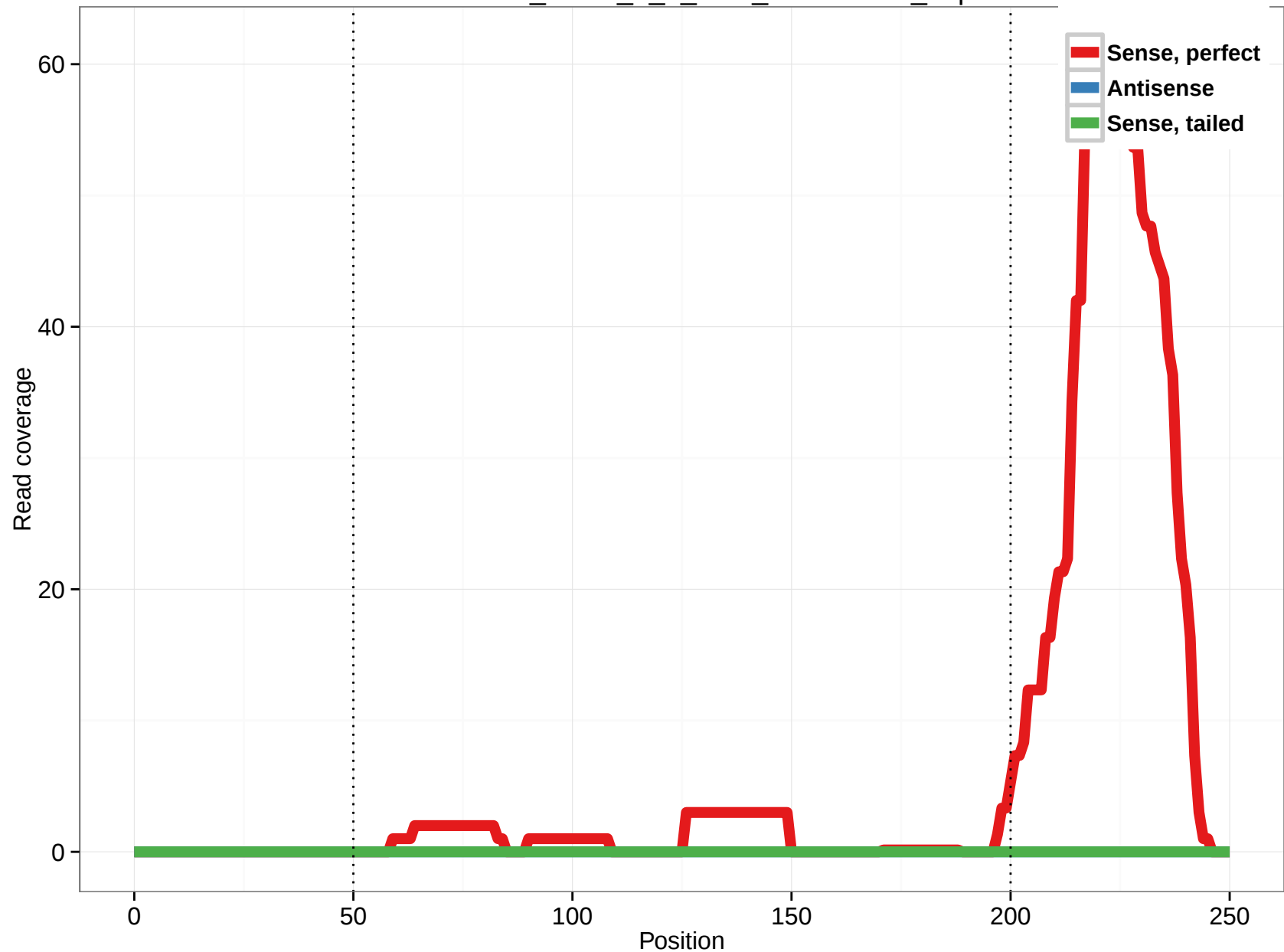
uc002tbc.2_intron_2_0_chr2_102407239_f.3p
