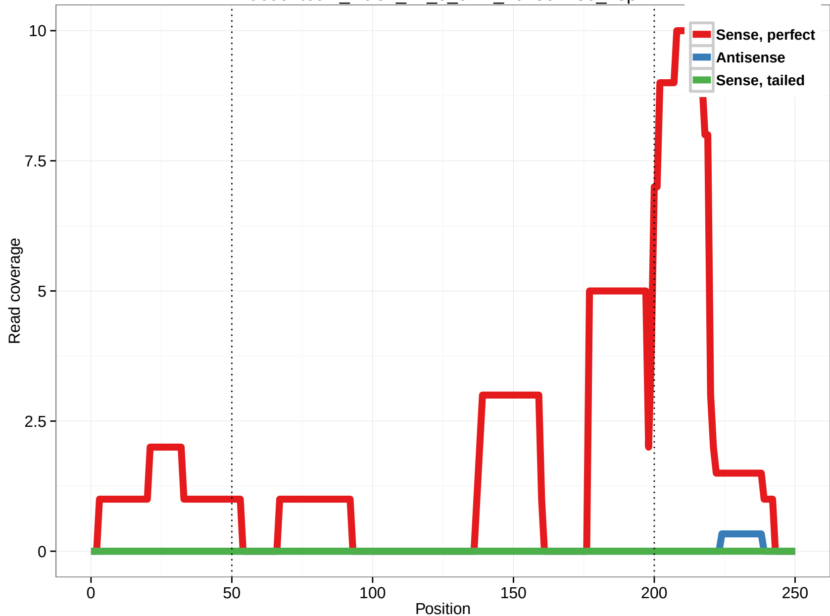
uc002tbc.2_intron_27_0_chr2_102501750_f.3p
