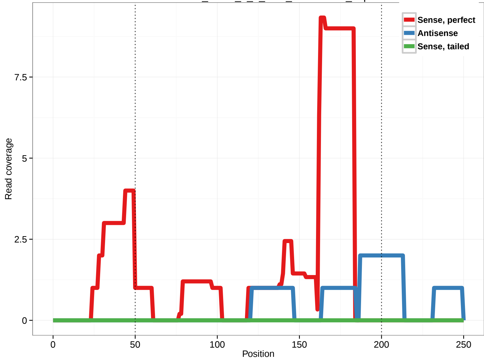
uc002taw.3_intron_3_0_chr2_101881510_f.5p
