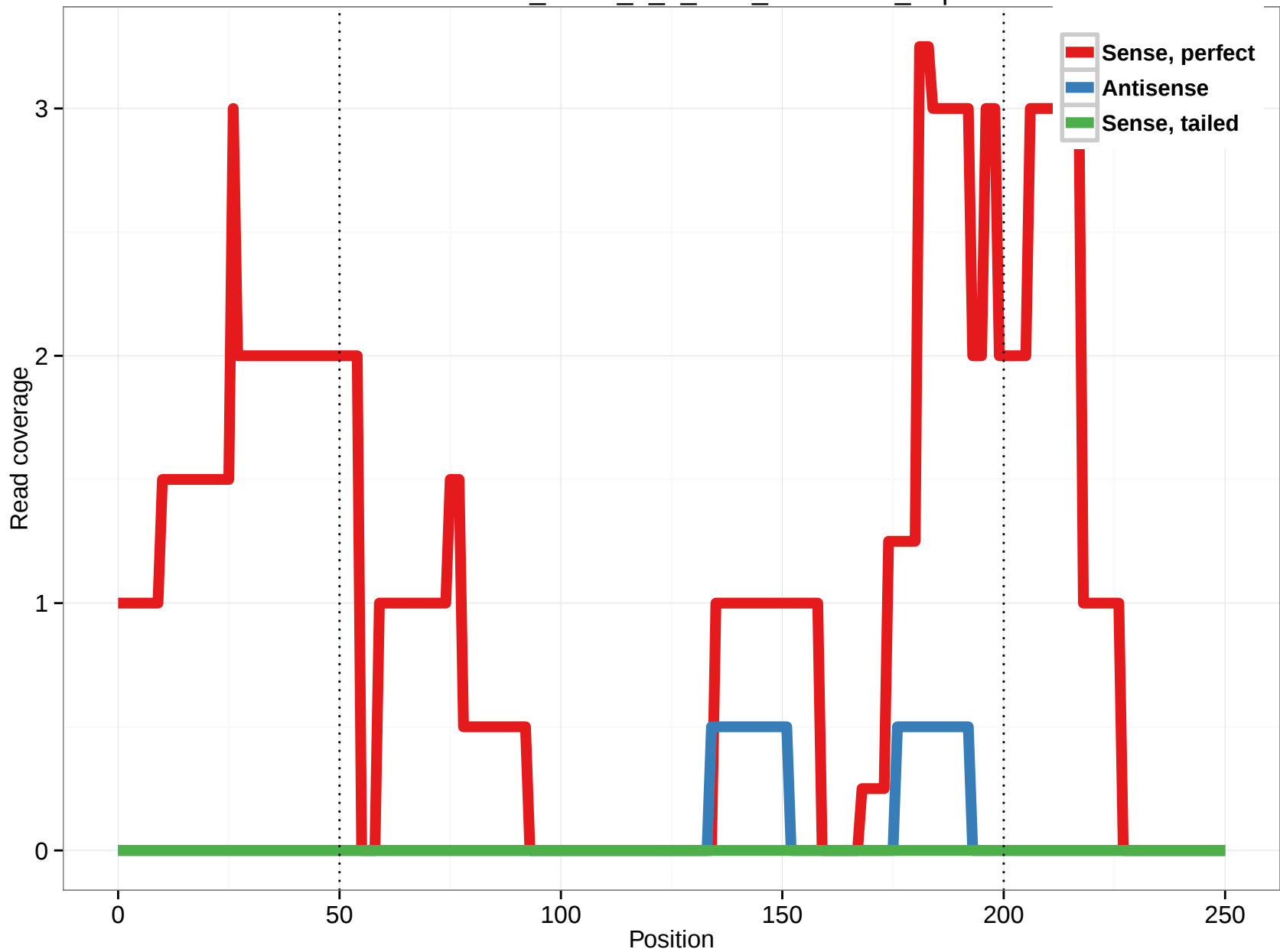
uc002ssx.3_intron_1_0_chr2_88470827_f.5p
