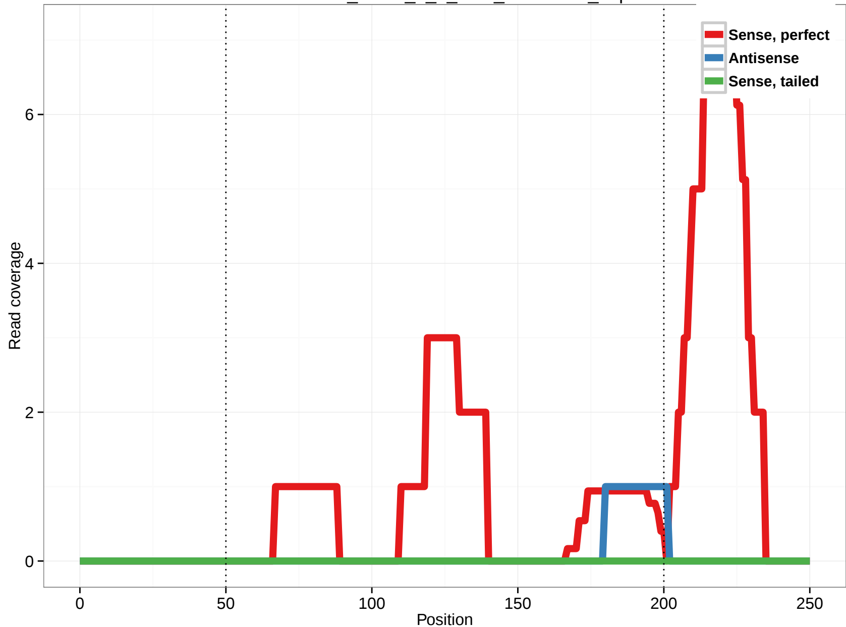
uc002sri.3_intron_4_0_chr2_86682311_f.3p
