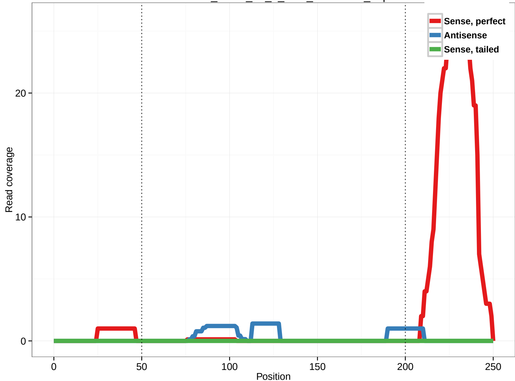
uc002sri.3_intron_10_0_chr2_86697532_f.3p
