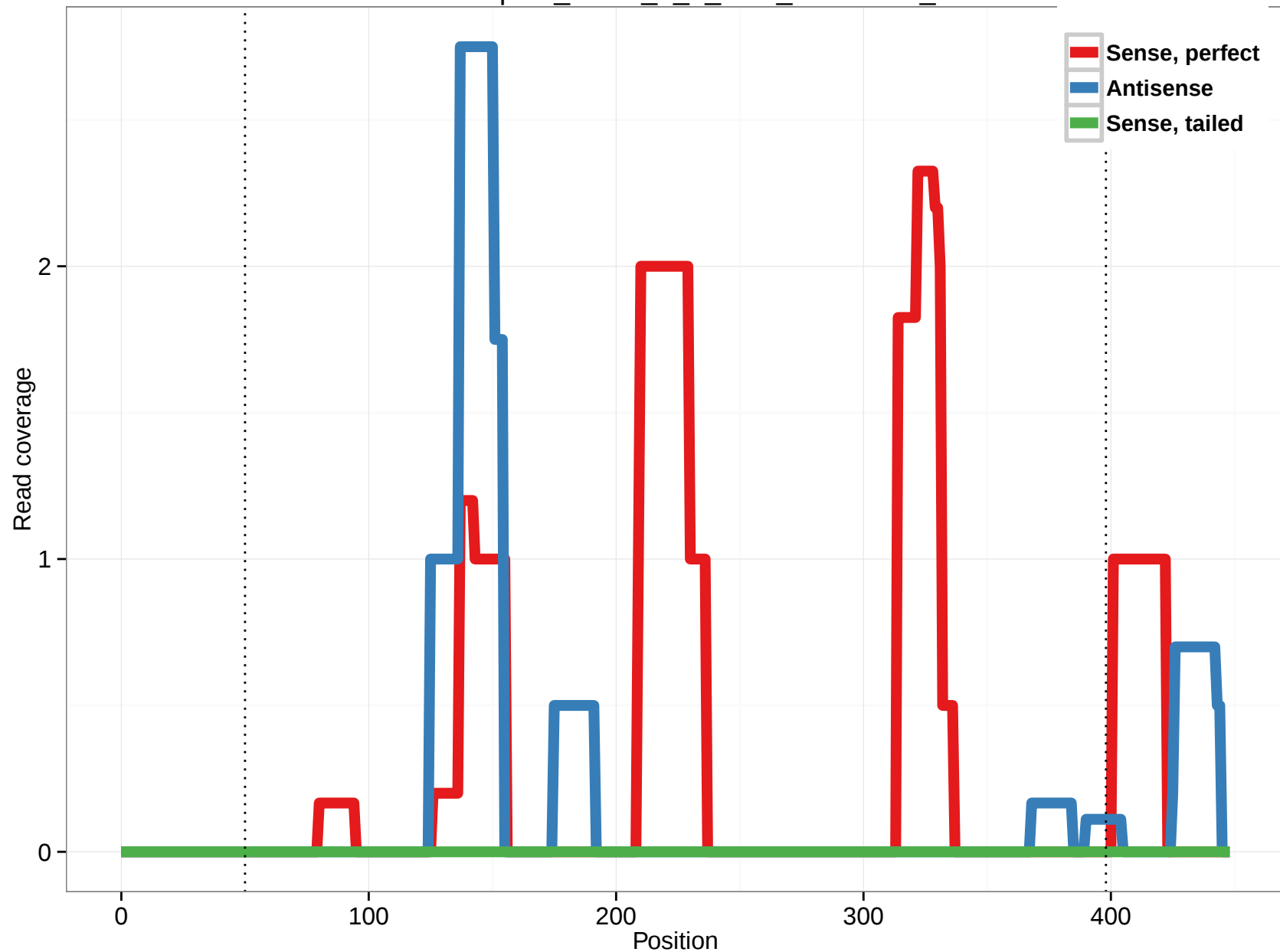
uc002spo.2_intron_8_0_chr2_85657139_f
