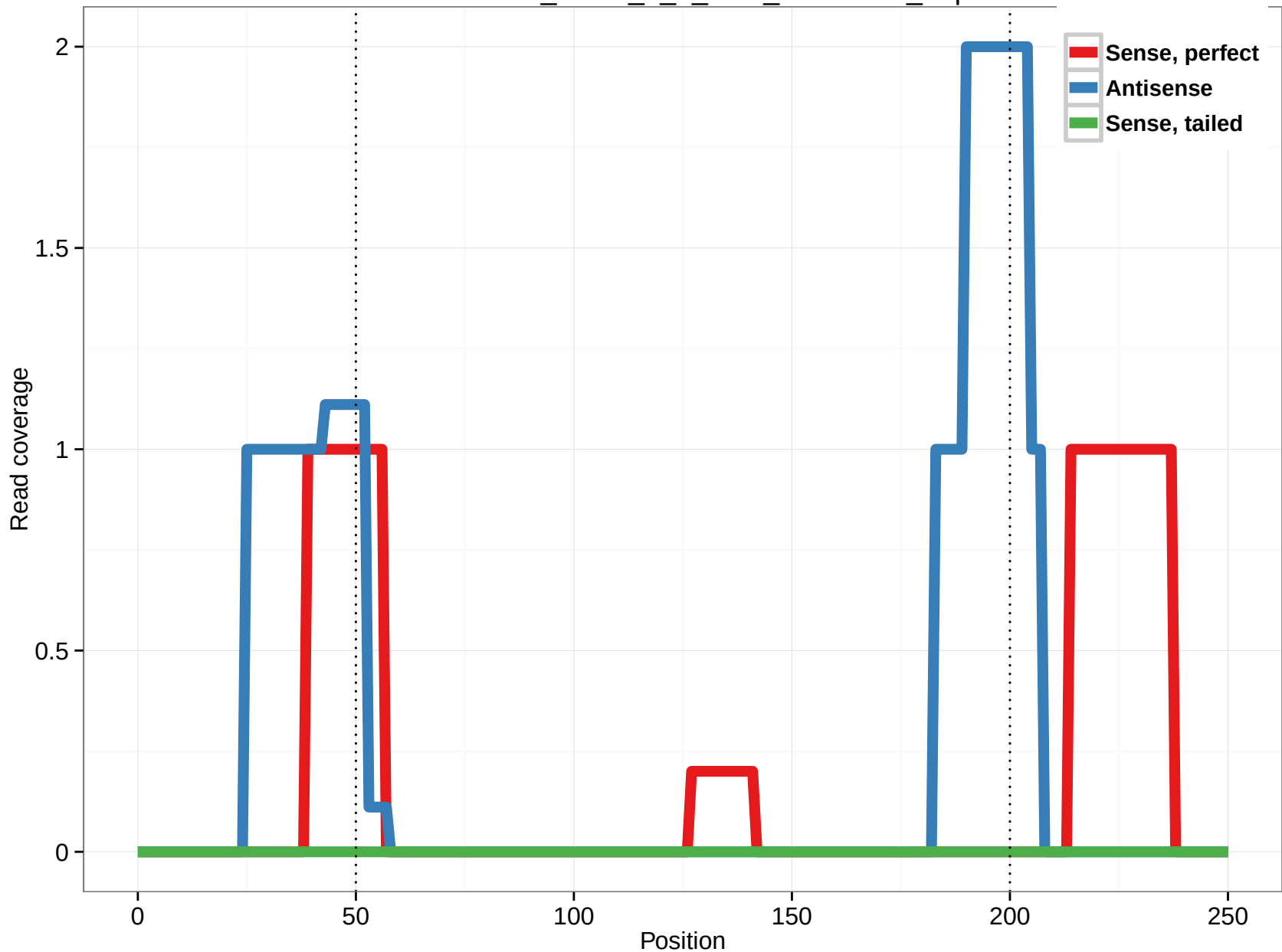
uc002snv.3_intron_1_0_chr2_78712979_r.5p
