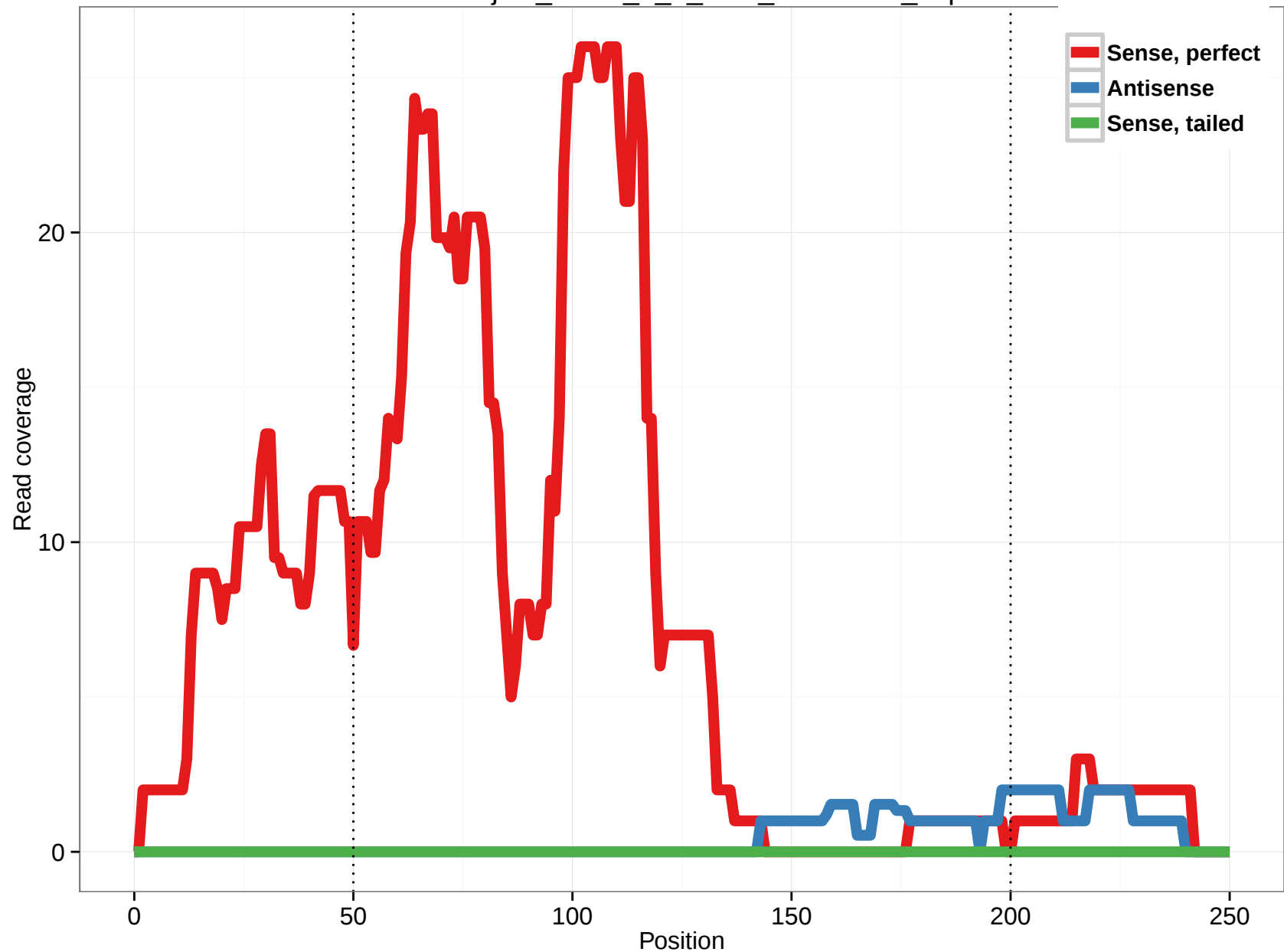
uc002sjs.2_intron_0_0_chr2_74056124_f.5p
