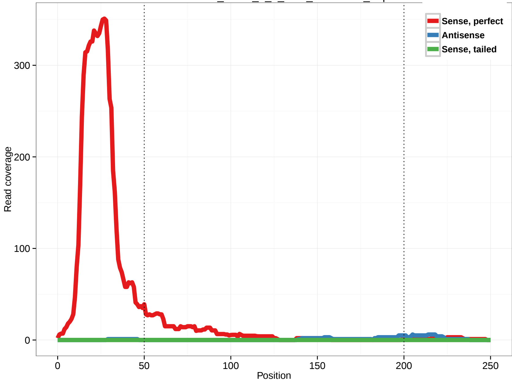
uc002shs.2_intron_1_0_chr2_71351674_r.5p
