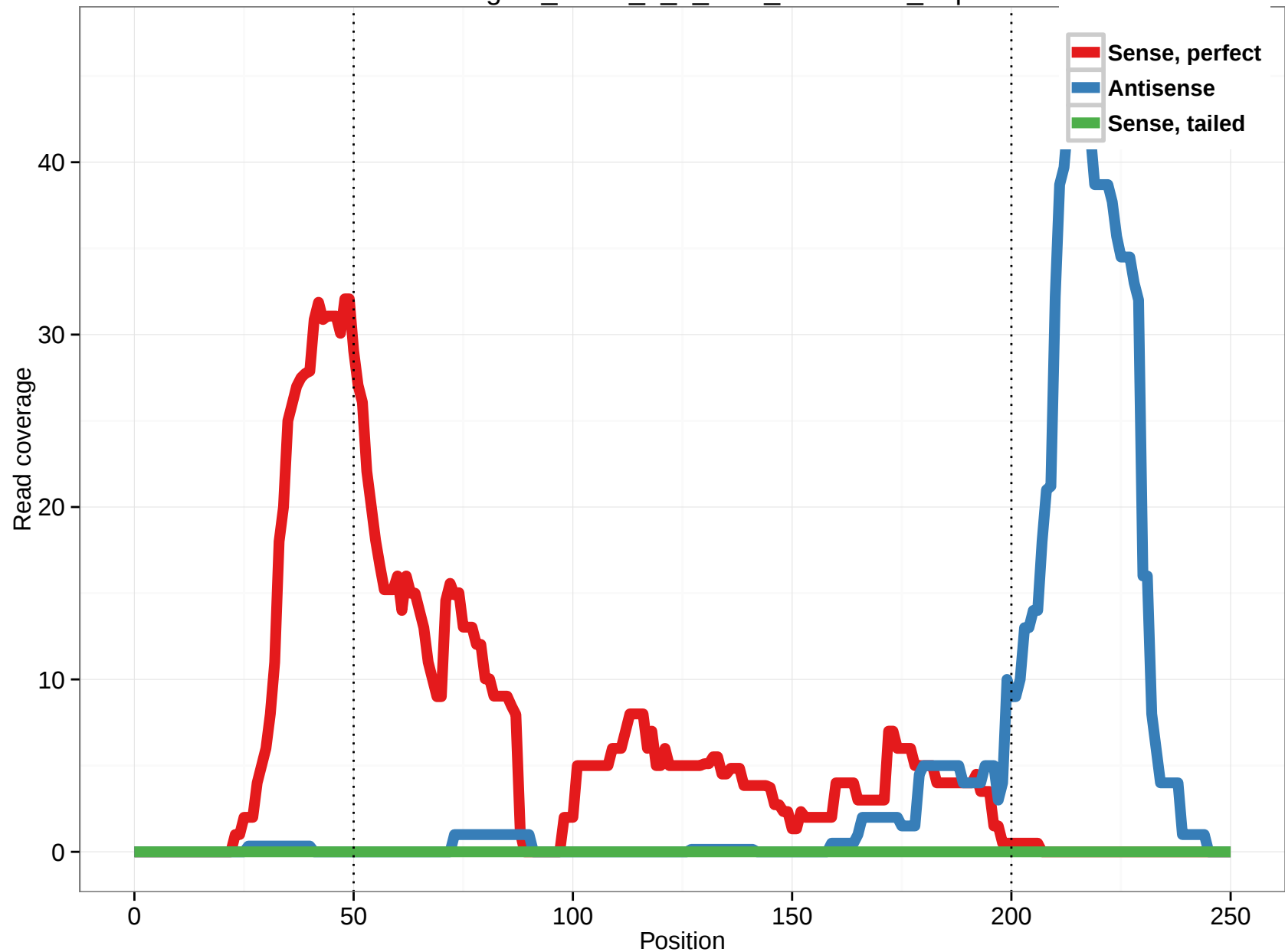
uc002sgh.2_intron_8_0_chr2_70410068_r.5p
