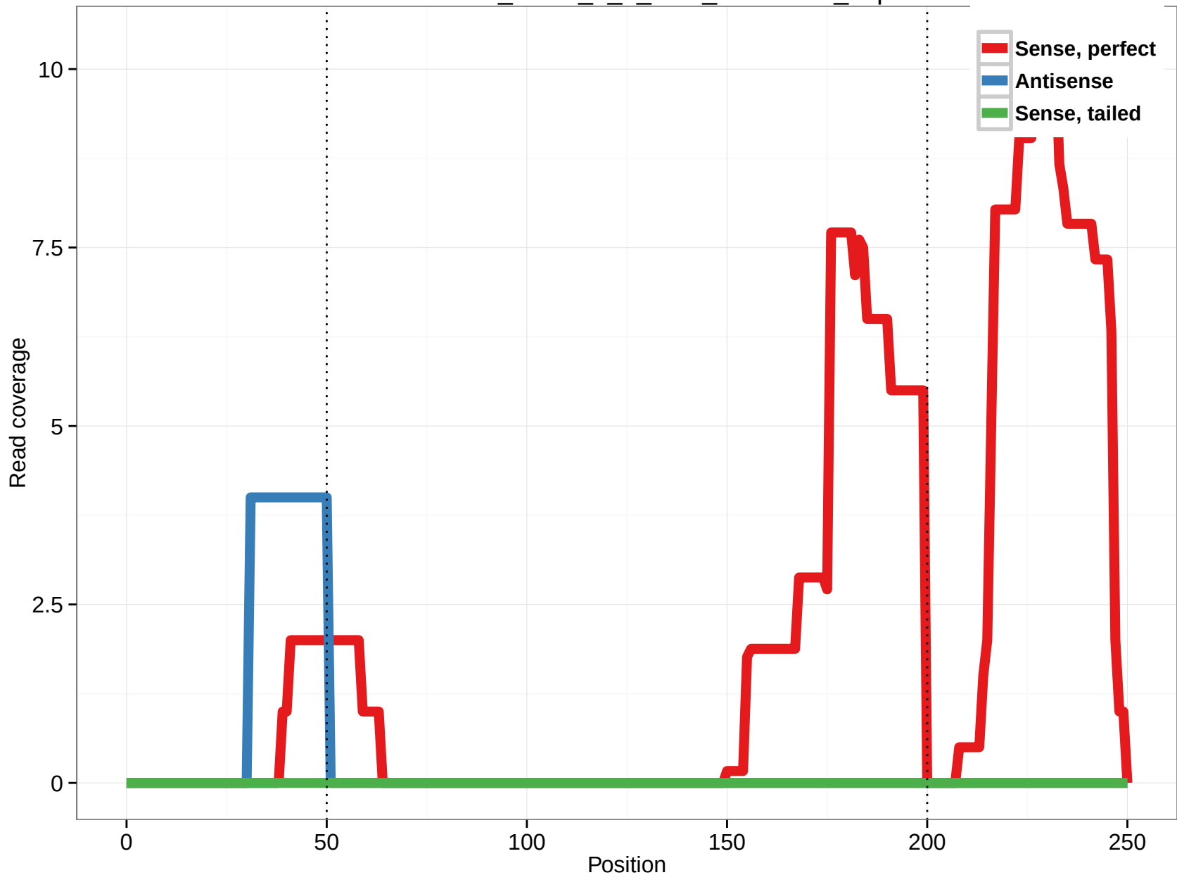
uc002sen.3_intron_2_0_chr2_68608037_f.3p
