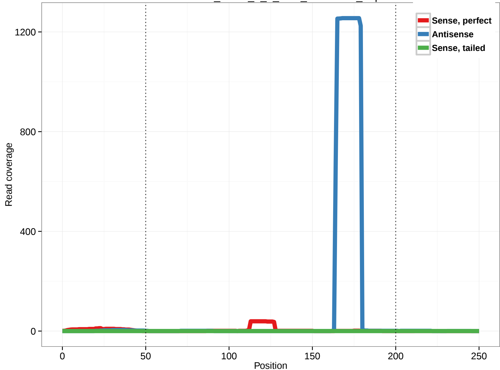
uc002sei.1_intron_4_0_chr2_68444264_r.5p
