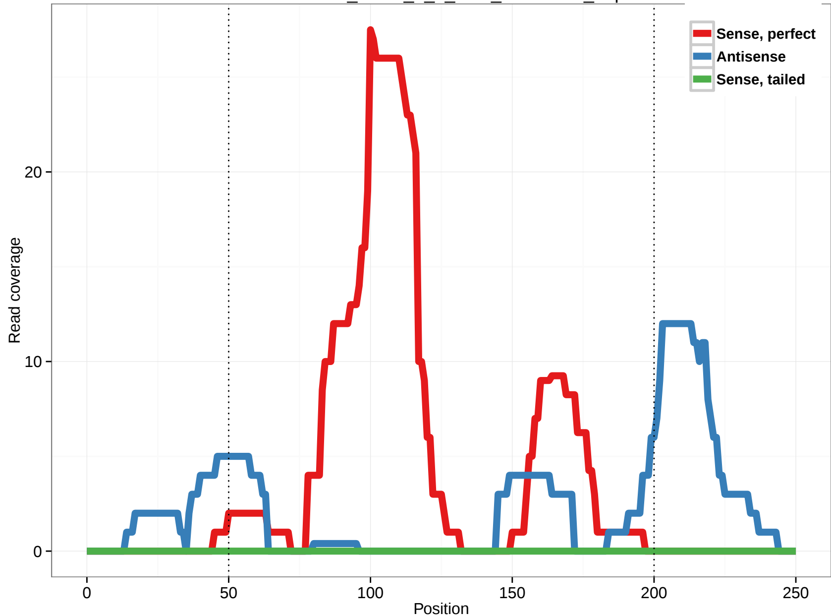
uc002sal.1_intron_1_0_chr2_61084056_r.5p
