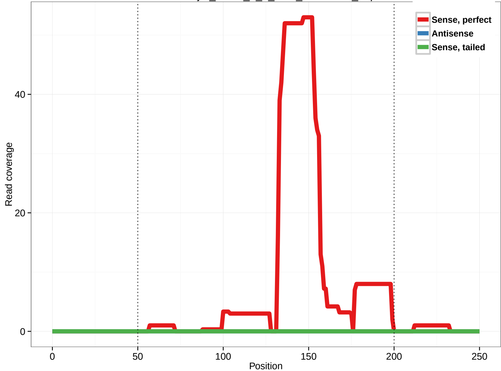
uc002saj.2_intron_8_0_chr2_61006911_f.3p
