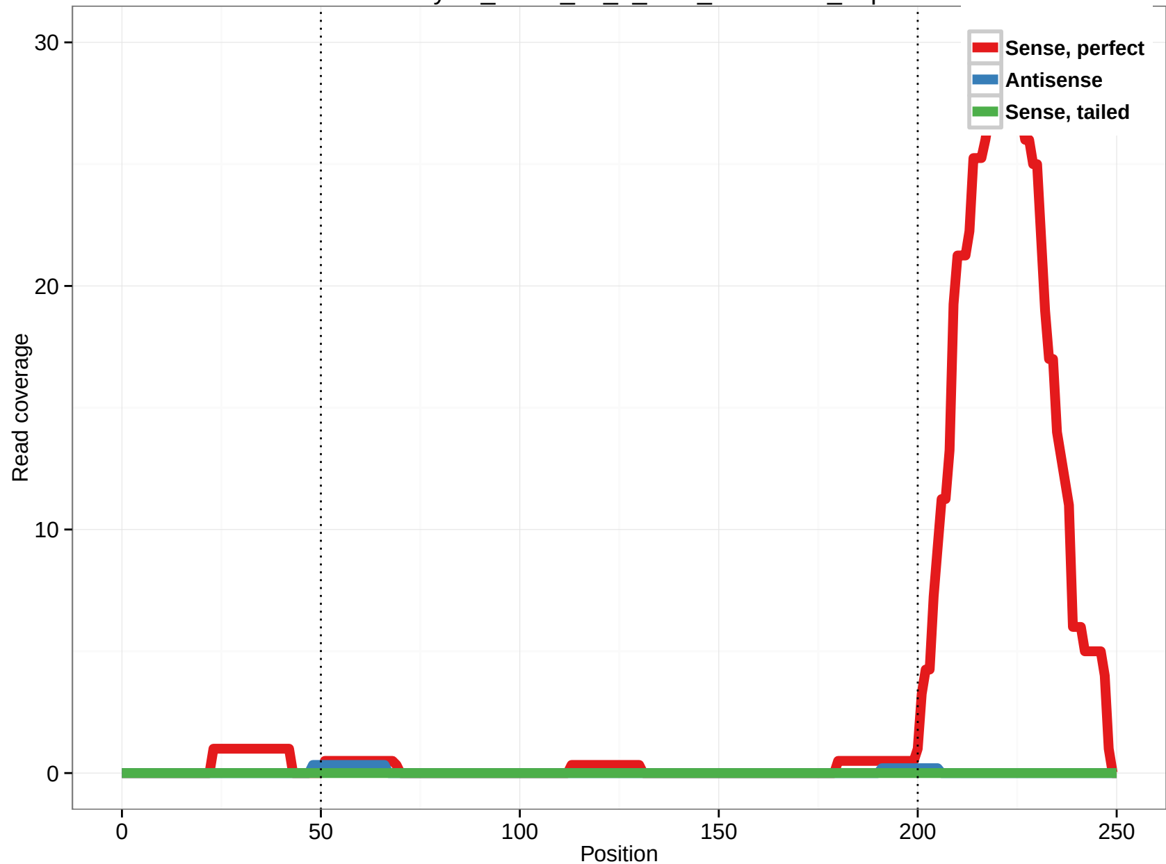
uc002ryv.2_intron_24_0_chr2_55576736_r.3p
