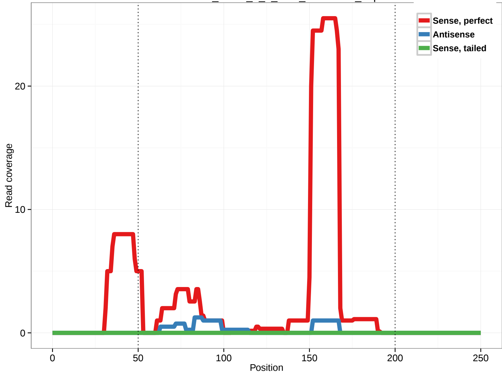
uc002rmv.2_intron_0_0_chr2_29338532_f.5p
