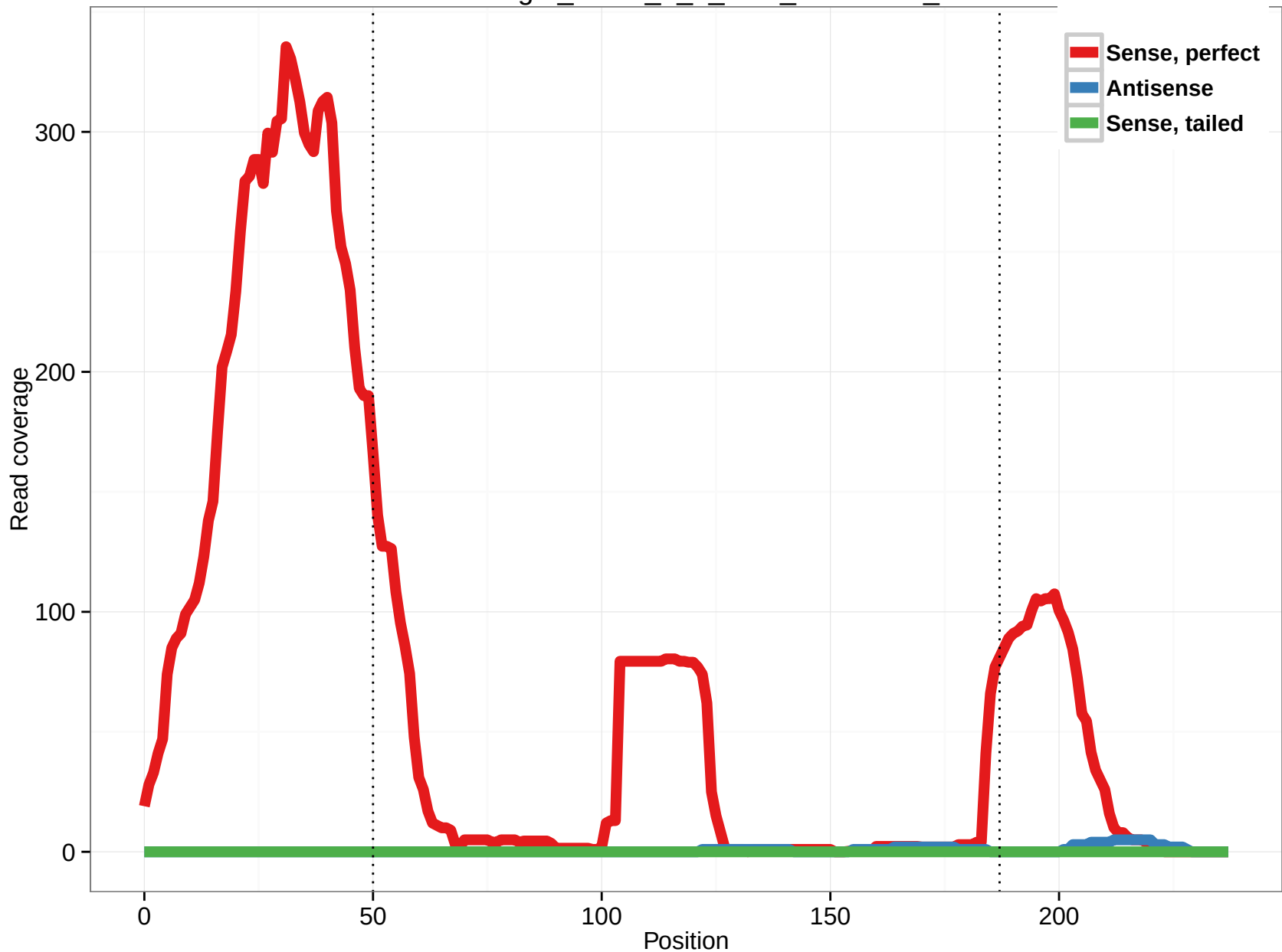
uc002rig.2_intron_1_0_chr2_27294332_r
