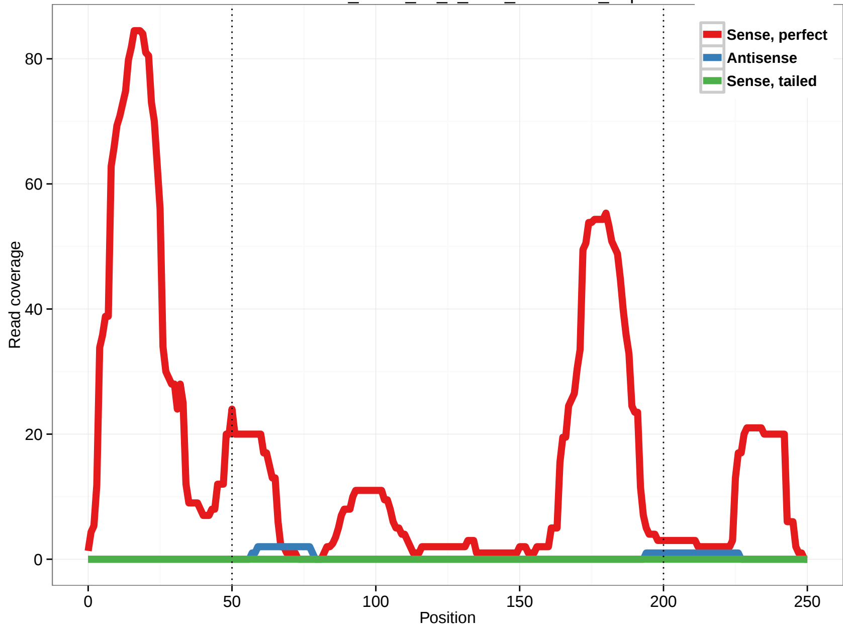
uc002rhb.1_intron_13_0_chr2_26540431_r.5p
