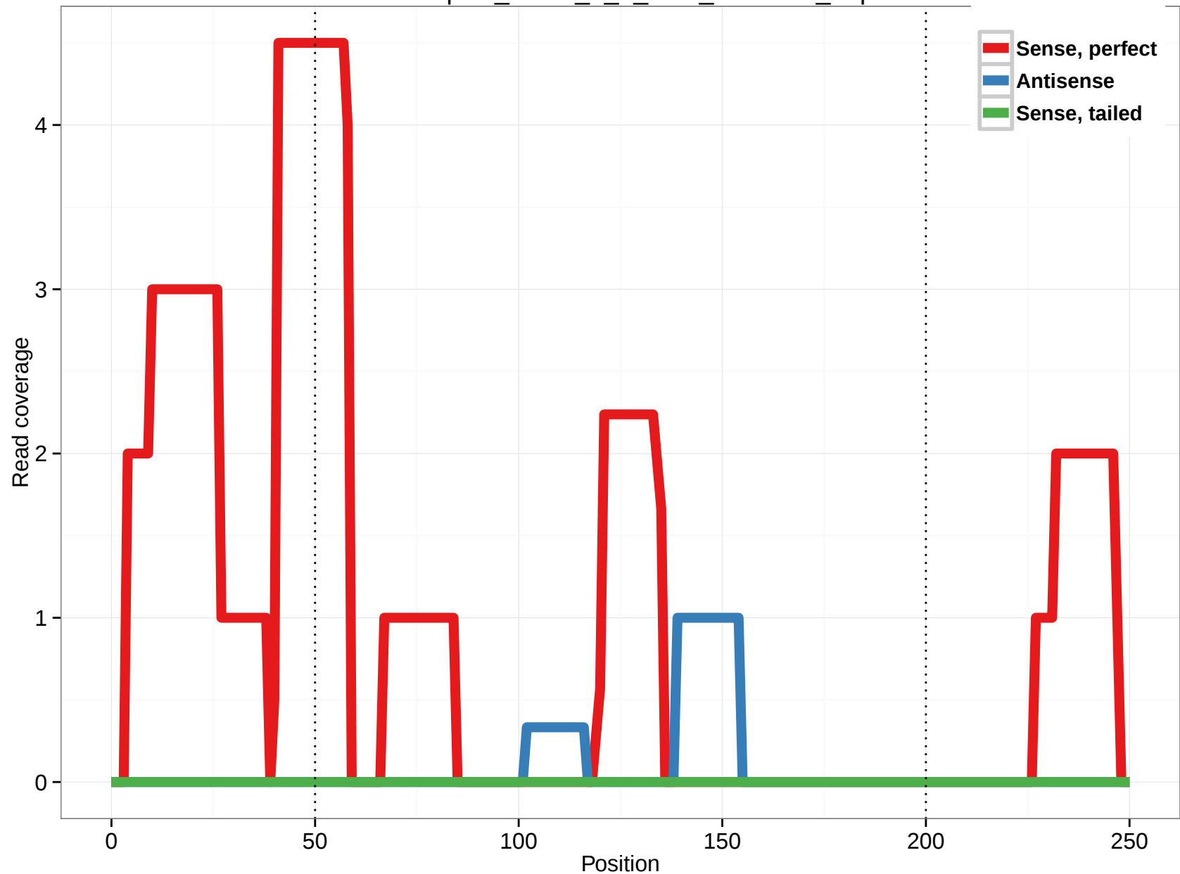
uc002qxt.2_intron_6_0_chr2_3604495_r.5p
